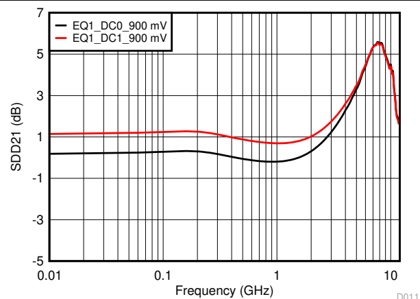
図 5-11. 900mV DC Gain Adjustment Curves
