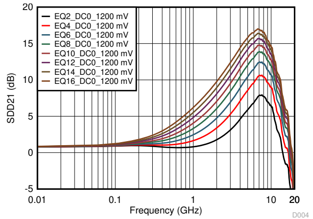
図 5-4. 1200mV DC0 Even EQ Settings Curves
