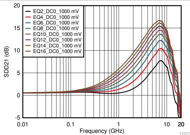
図 5-7. 1000mV DC0 Gain Even EQ Settings Curves
