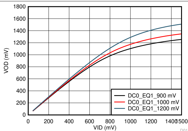
図 5-14. 5GHz Sine Wave VID vs VOD Linearity Range Setting
