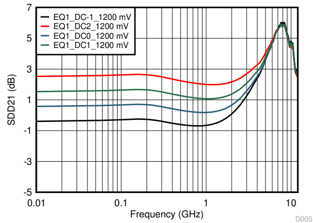
図 5-5. 1200mV DC Gain Adjustments Curves
