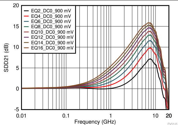
図 5-10. 900mV DC0 Gain Even EQ Settings Curves
