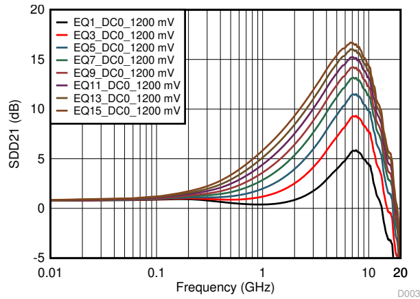
図 5-3. 1200mV DC0 Gain Odd EQ Settings Curves
