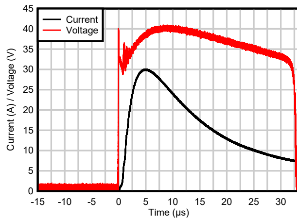
図 6-1. 8/20 \mu s Surge Response
