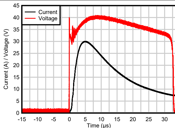
図 5-1. 8/20 \mu s Surge Response
