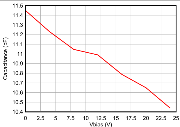
図 5-2. Capacitance vs Bias Voltage
