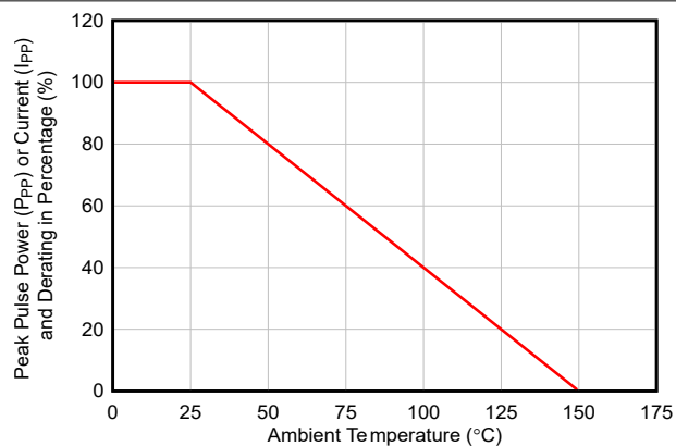
図 5-8. Peak Pulse Power Derating Curve
