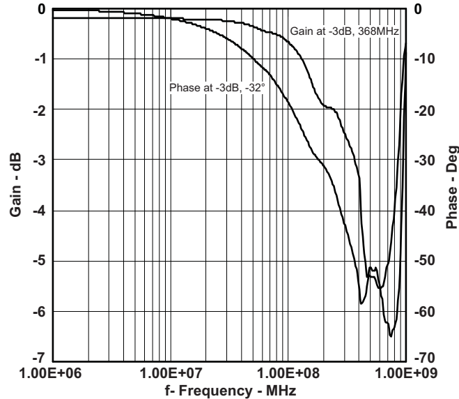
Figure 3. Frequency Response
