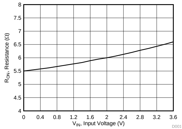
⊠ 1. ON-Resistance vs Input Voltage
