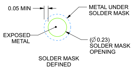
SOLDER MASK DETAILS NOT TO SCALE
