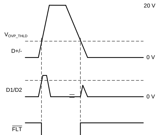
16. Overvoltage Protection Waveform, 20 V
