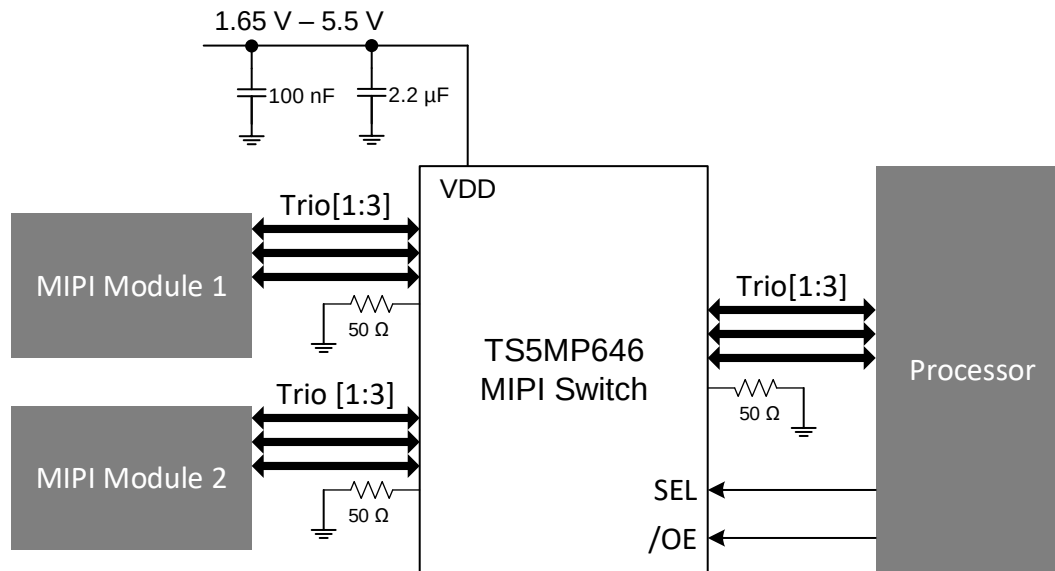
FIG 25. Typical C-PHY Application
