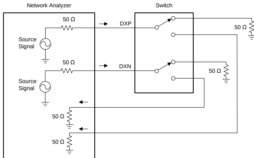
FIG 12. Off Isolation
