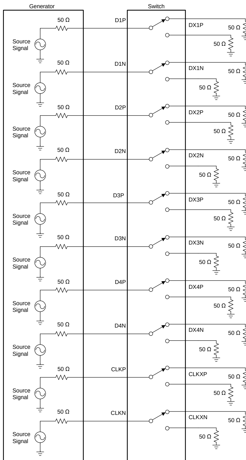
FIG 15. t_{PD} , t_{SKEW(INTRA)} and t_{SKEW(INTER)} Setup
