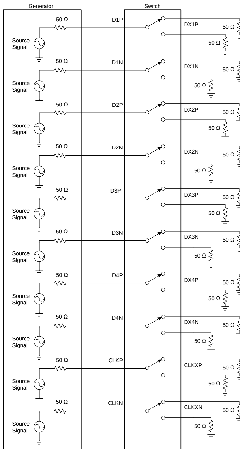
FIG 15. t_{PD} , t_{SKEW(INTRA)} and t_{SKEW} Setup
