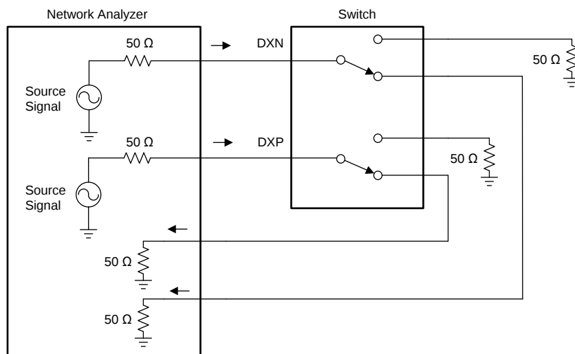
FIG 14. BW and Insertion Loss
