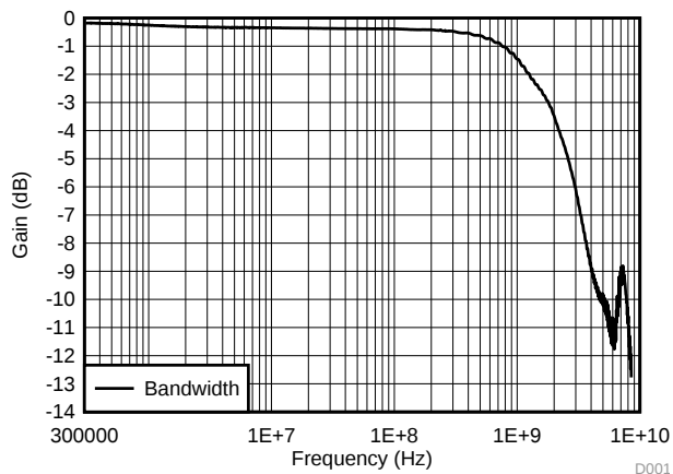
⊠ 25. Differential Bandwidth
