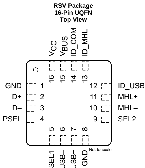
Pin Functions
