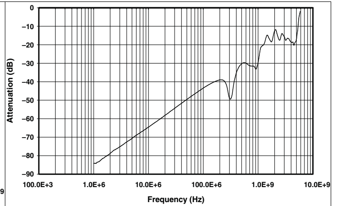
Figure 2. OFF Isolation
