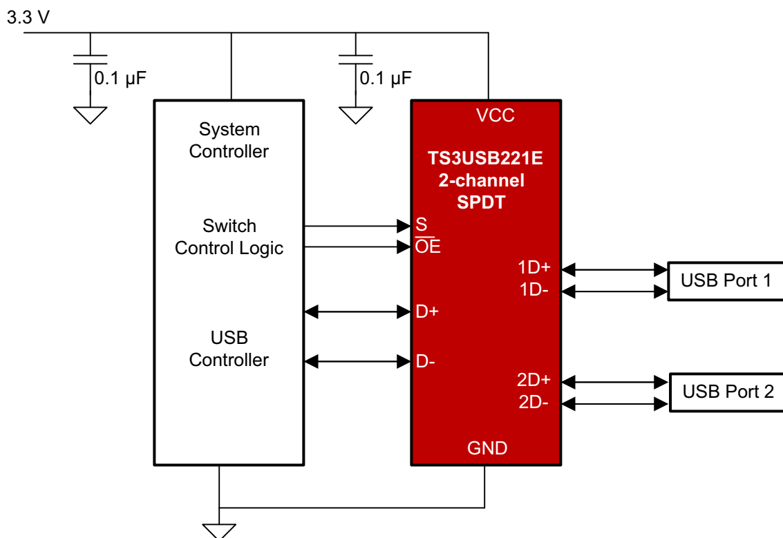
図 7-1. Simplified Schematic
