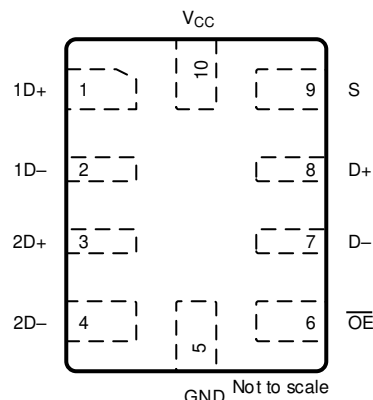
図 4-2. RSE Package, 10-Pin UQFN (Top View)
