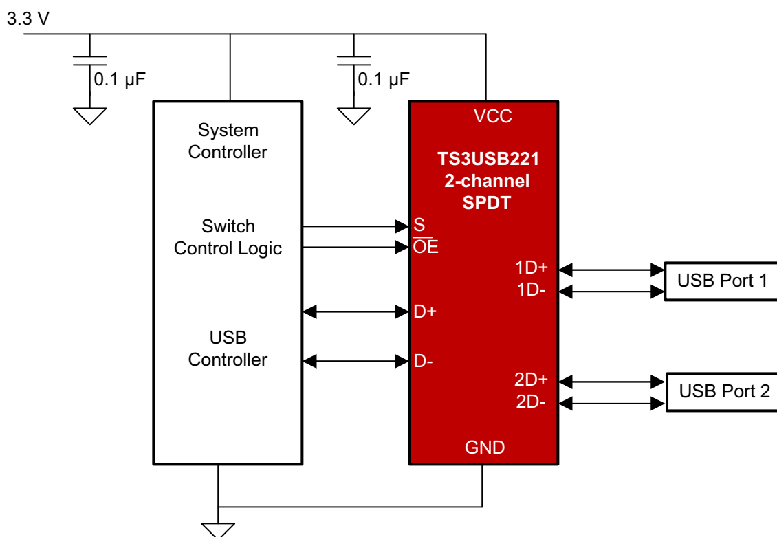
図 8-1. Simplified Schematic
