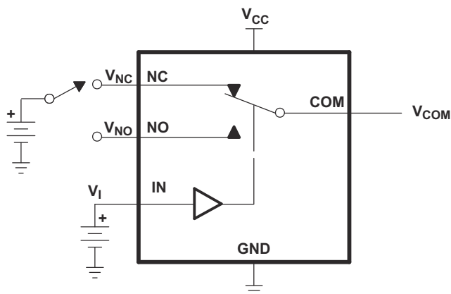
7-3. ON-State Leakage Current ( I_{COM(ON)} , I_{NC(ON)} , I_{NO(ON)} )
