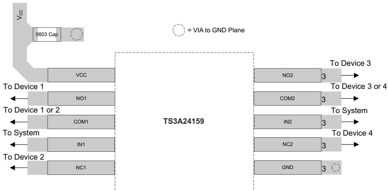
✎ 11-1. Layout Example
