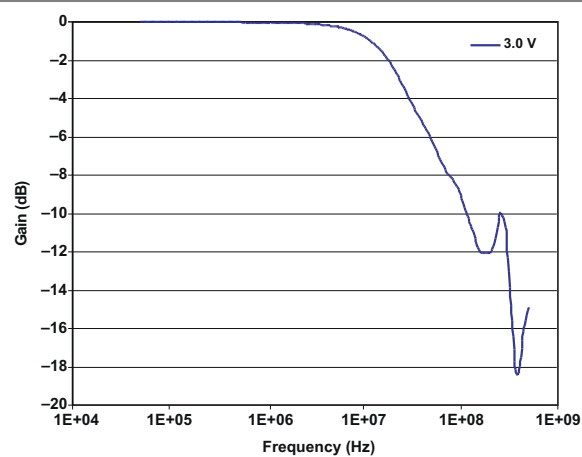
Figure 6-6. Bandwidth
