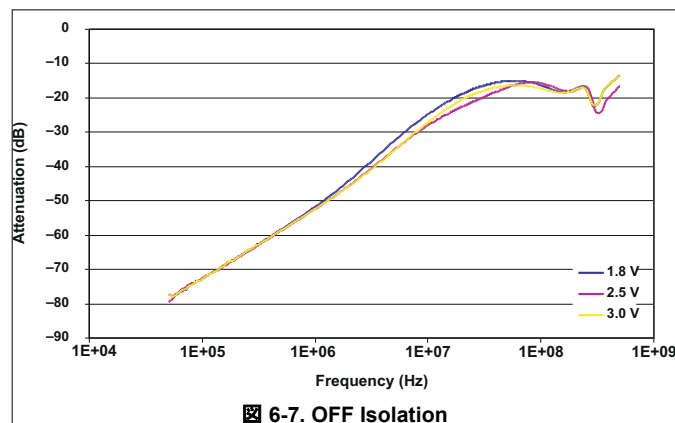
FIG 6-7. OFF Isolation
