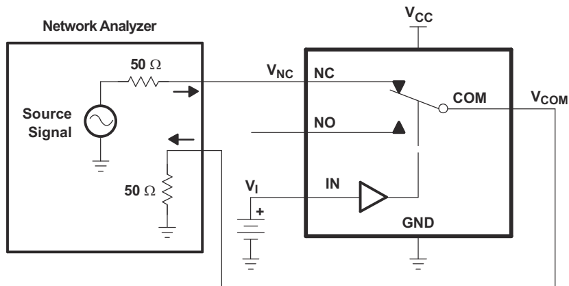
7-7. Bandwidth (BW)
