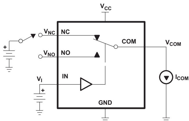
7-1. ON-State Resistance
