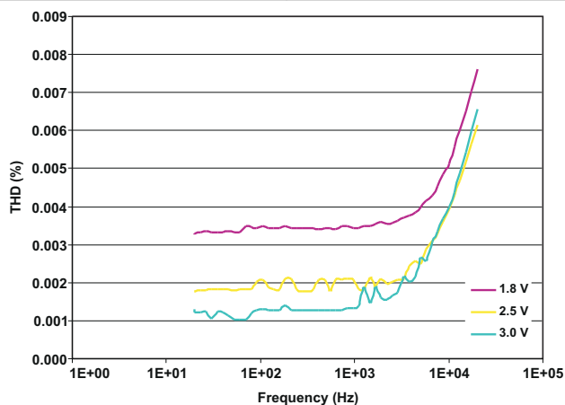
FIG 6-9. Total Harmonic Distortion vs Frequency
