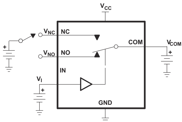
7-2. OFF-State Leakage Current ( I_{NC(OFF)} , I_{NC(PWROFF)} , I_{NO(OFF)} , I_{NO(PWROFF)} , I_{COM(OFF)} , I_{COM(PWROFF)} )
