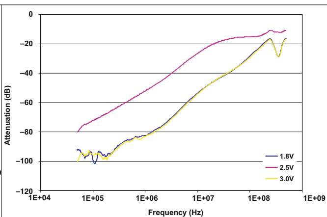
FIG 6-8. Crosstalk
