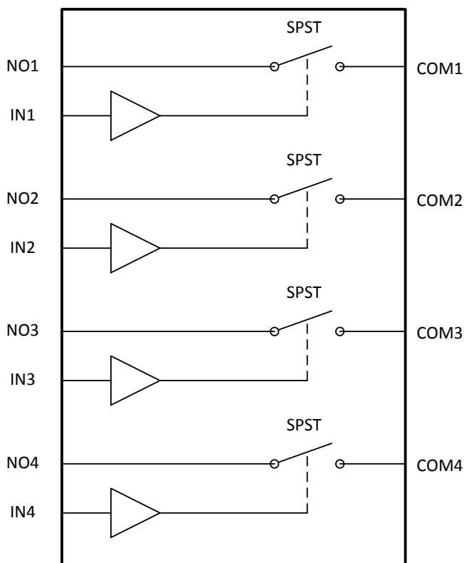
Simplified Schematic
