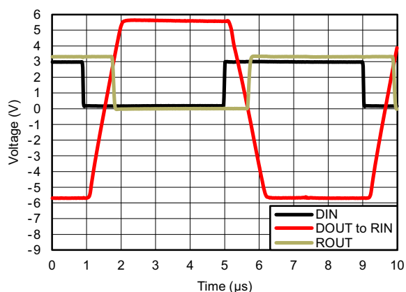
図 9-2. 250 kbps Driver to Receiver Loopback Timing Waveform, V_{CC} = 3.3 V
