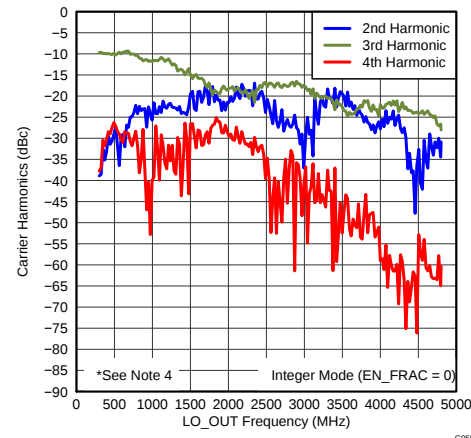
Figure 60. LO Harmonics
