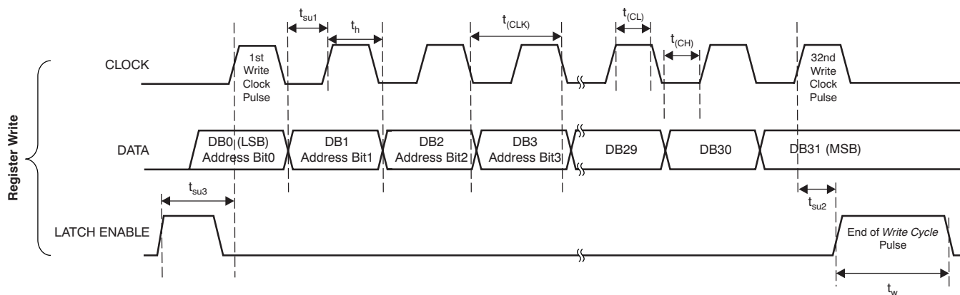
Figure 1. 4WI Timing Diagram
