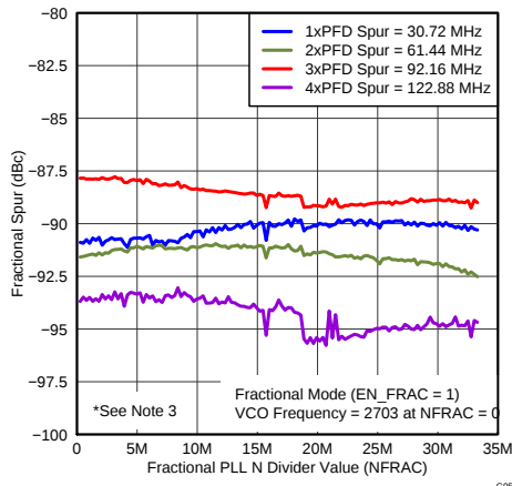
Figure 59. Multiples of PFD Spurs (Fractional Mode)
