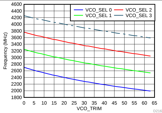
Figure 106. Frequency vs VCO_TRIM
