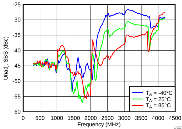
Figure 44. Unadjustable SBS vs Temperature, Typical Operating Mode
