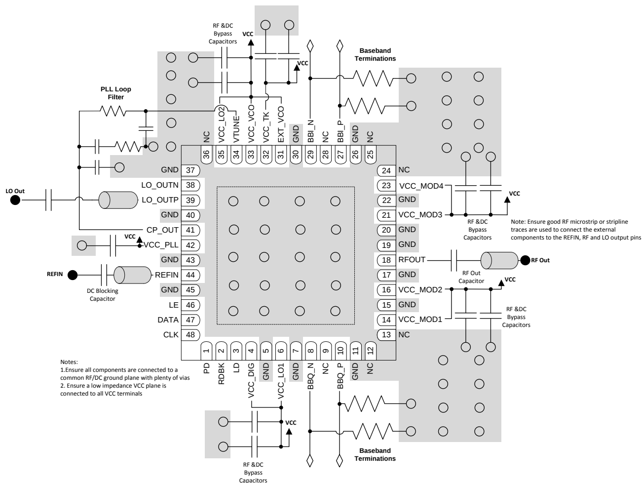
Figure 139. Layout
