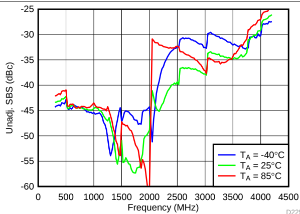
Figure 46. Unadjustable SBS vs Temperature, High Gain Mode
