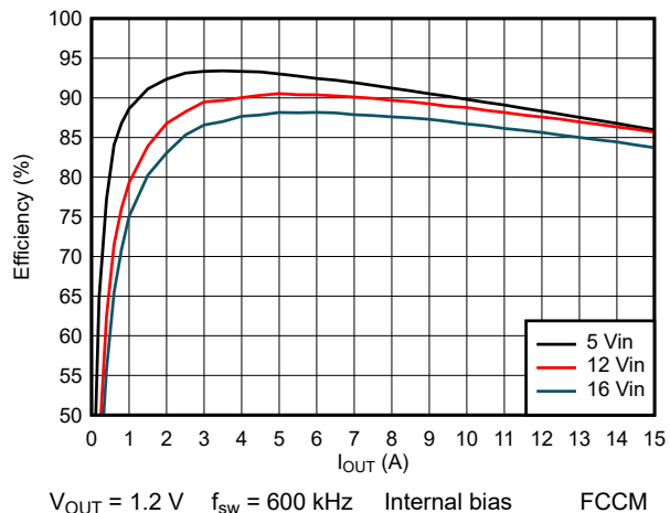
图 8-5. Efficiency
