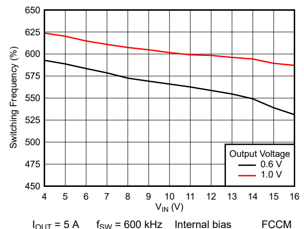
图 8-21. Switching Frequency
