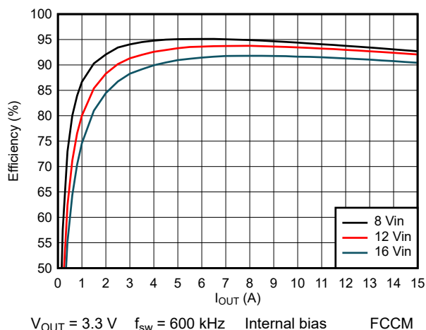
图 8-8. Efficiency
