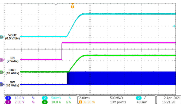
I_{OUT} = 15\text{ A} FCCM 8-34. Startup Through Enable
