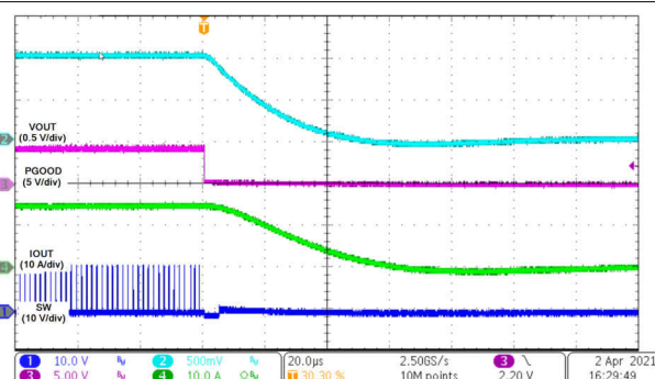
I_{OUT} = 15\text{ A} FCCM 8-36. Shutdown Through Enable
