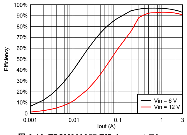
Figure 6-16. TPSM863257 Efficiency at 5V OUT
