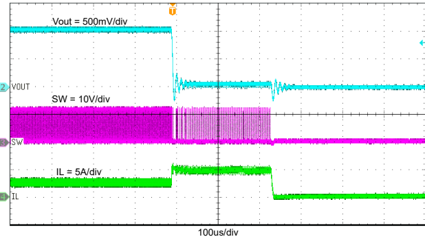
8-17. TPSM863252 Normal Operation to Output Hard Short
