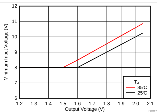
FIG 11. Minimum Input Voltage
