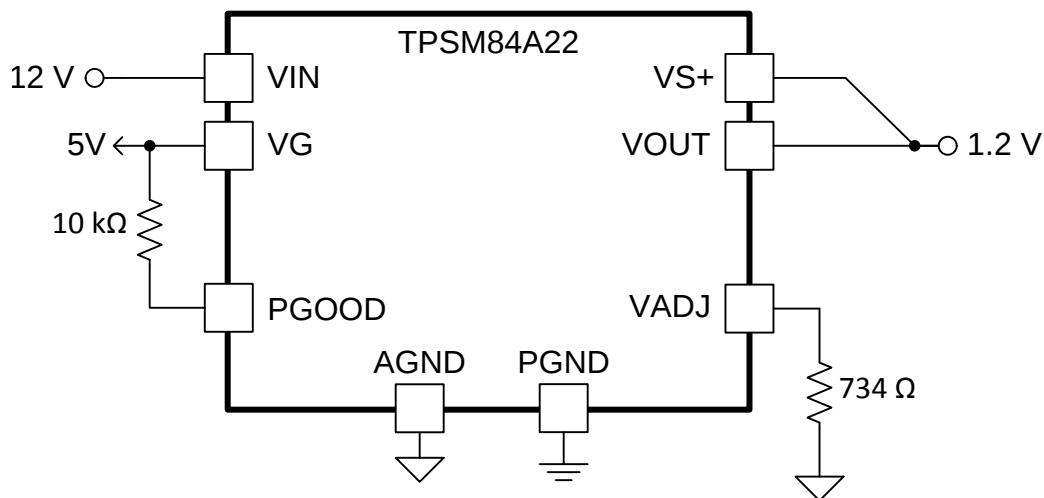
18. Typical Application Schematic
