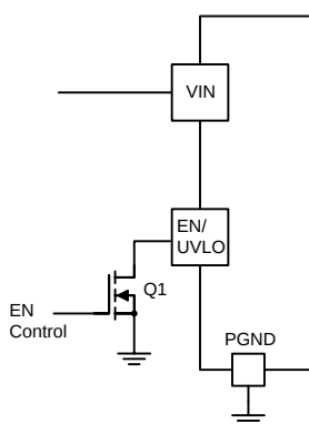
Figure 15. Enable Control
