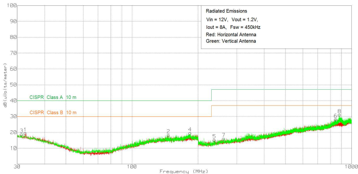
Figure 31. Radiated Emissions 12-V Input, 1.2-V Output, 8-A Load (EN55011 Class B)
