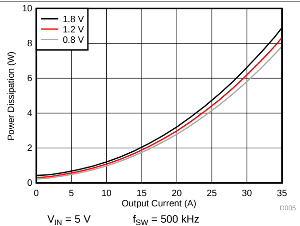
FIG 8. Power Dissipation vs Output Current
