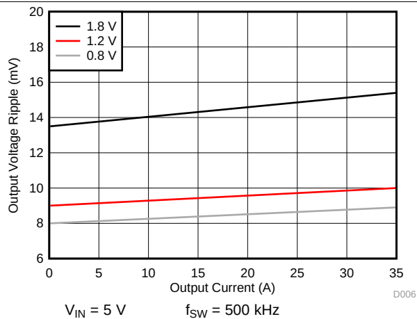
FIG 9. Voltage Ripple vs Output Current
