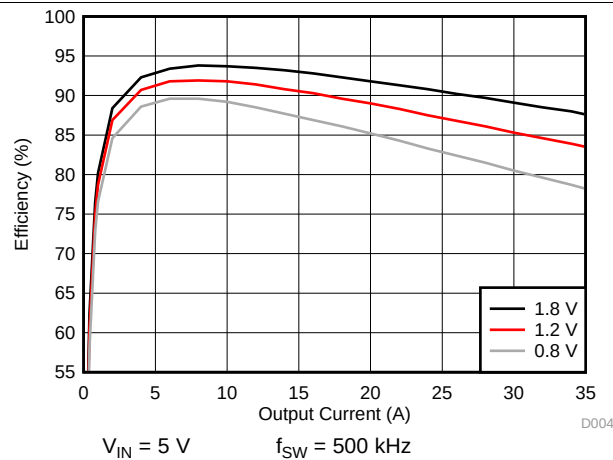
FIG 7. Efficiency vs Output Current
