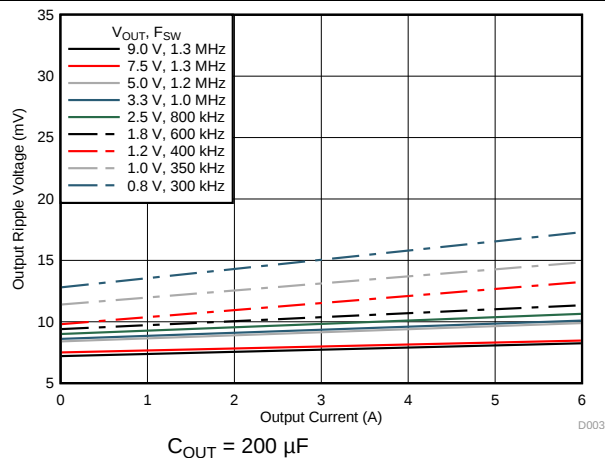
FIG 3. Ripple Voltage vs Output Current
