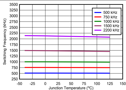
图 6-16. Switching Frequency vs Temperature
