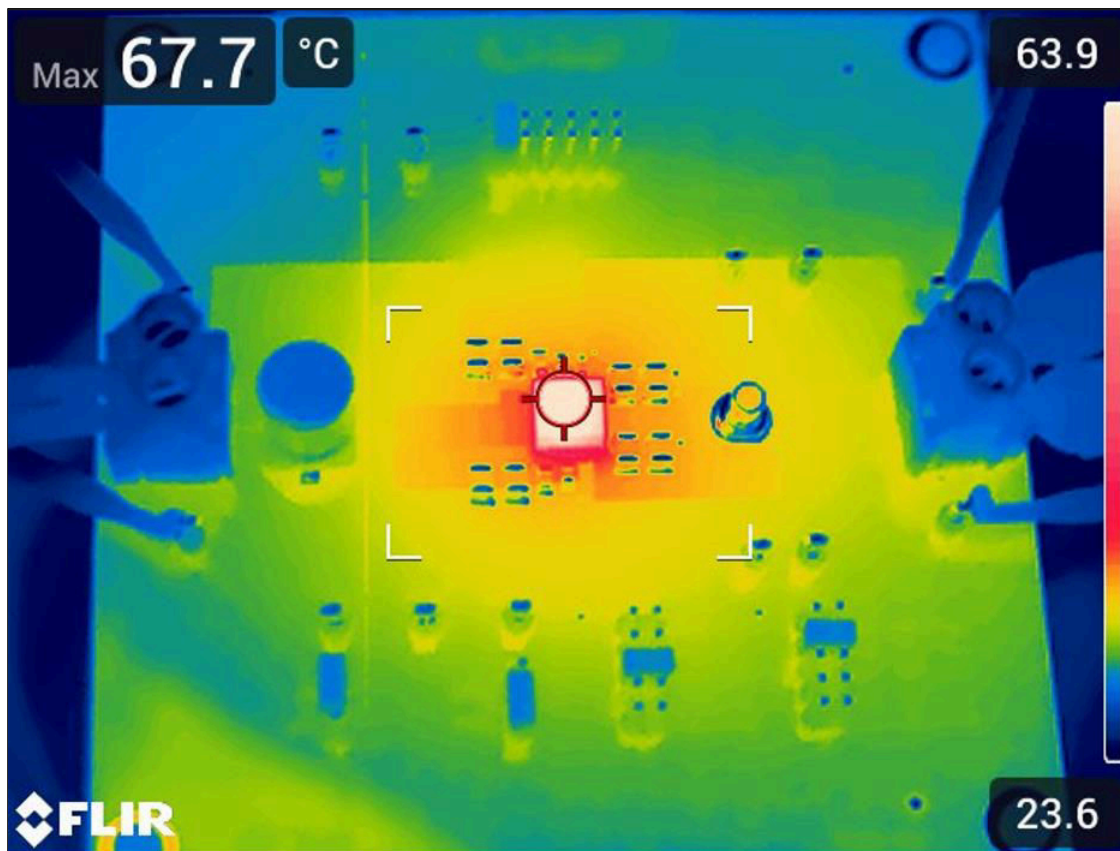
图 8-17. Thermal Image at 25^{\circ}\text{C} Ambient
