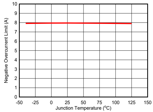
図 6-4. Negative Overcurrent Limit
