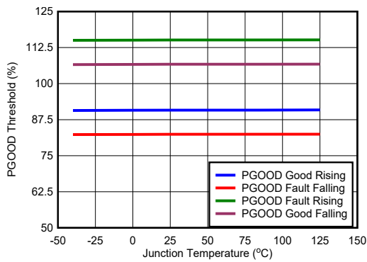
Figure 6-9. PG Threshold
