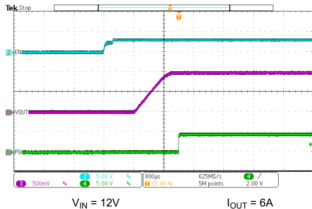
7-11. EN Start-Up – With Load
