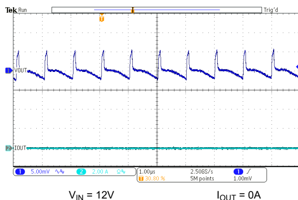
7-15. Output Ripple – No Load
