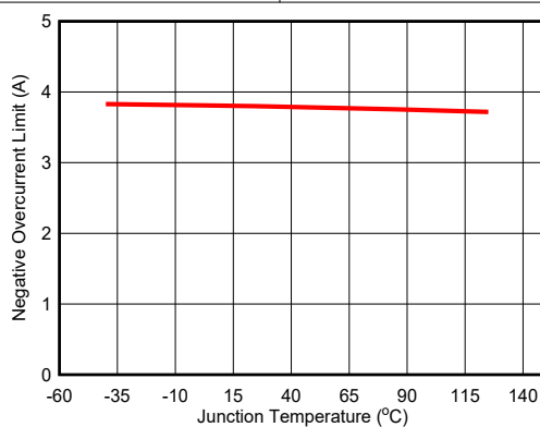
5-15. Negative Overcurrent
