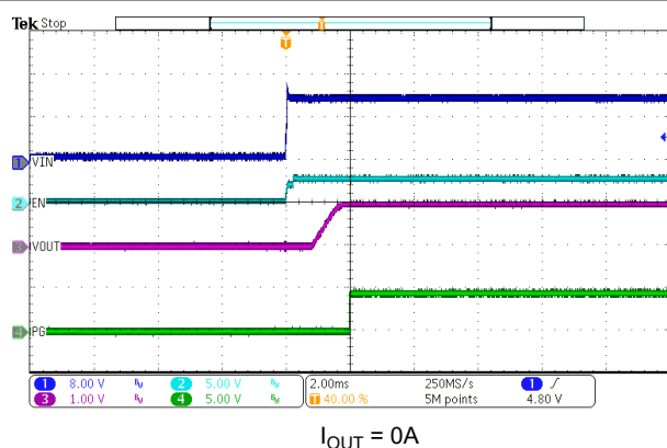
7-13. VIN Start-Up
