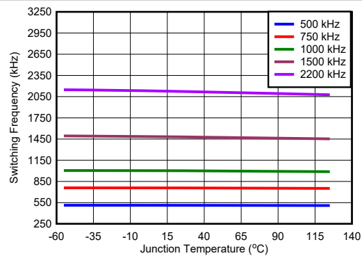
図 5-12. Switching Frequency
