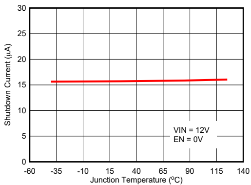
5-13. Shutdown Current
