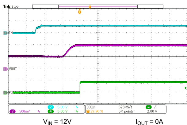
7-12. EN Start-Up – 0.5V Prebias
