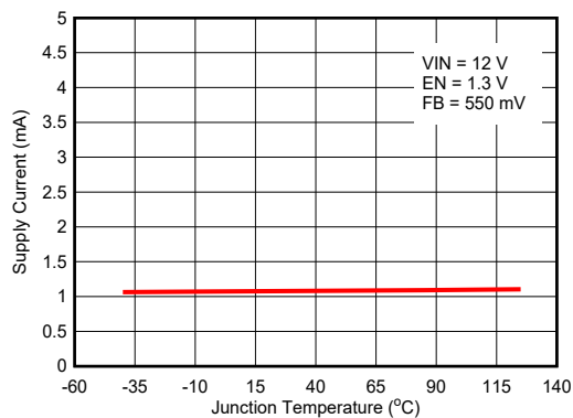
5-14. Non-Switching Supply Current
