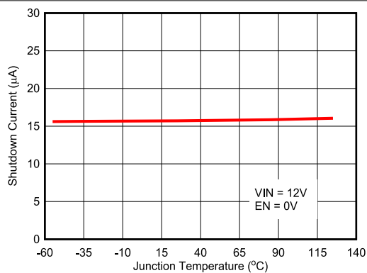
図 5-13. Shutdown Current
