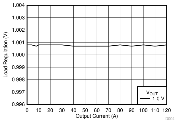
6-5. VOUTA Load Regulation
