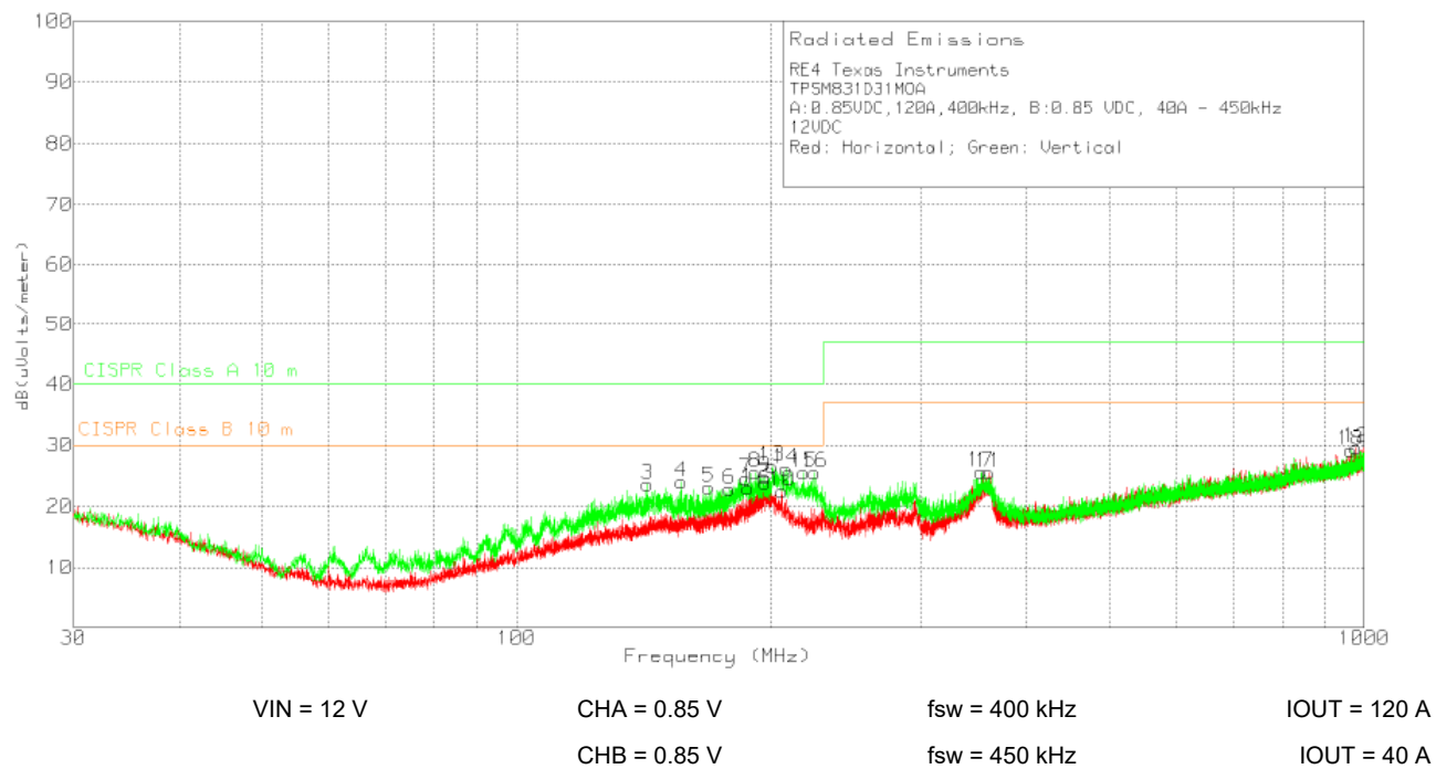
8-15. Radiated EMI
