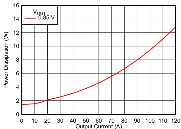
8-4. VOUTA Power Dissipation
