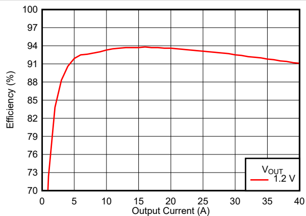
8-3. VOUTB Efficiency
