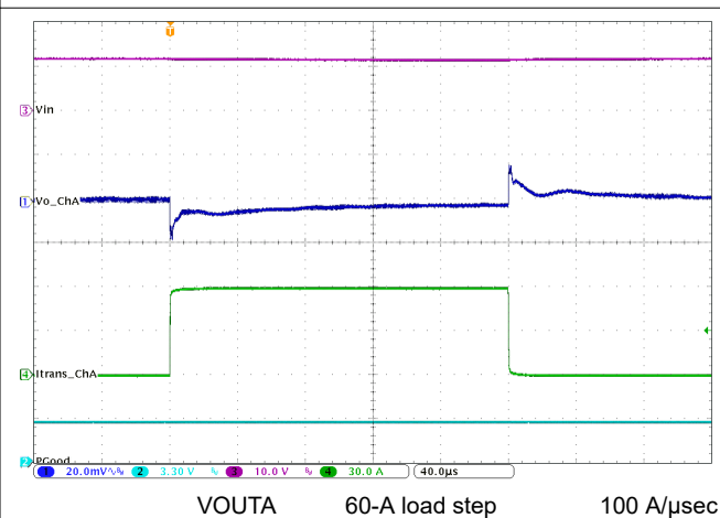
图 8-13. Transient Response
