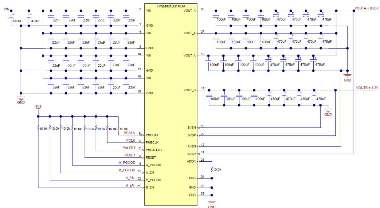
図 8-1. Typical Dual Output Schematic (Dual Outputs: VOUTA = 0.85V, 120A and VOUTB = 1.2V, 40A)
