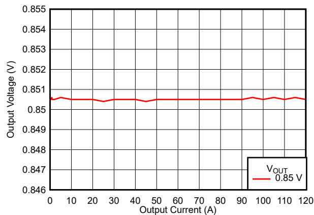
8-6. VOUTA Load Regulation
