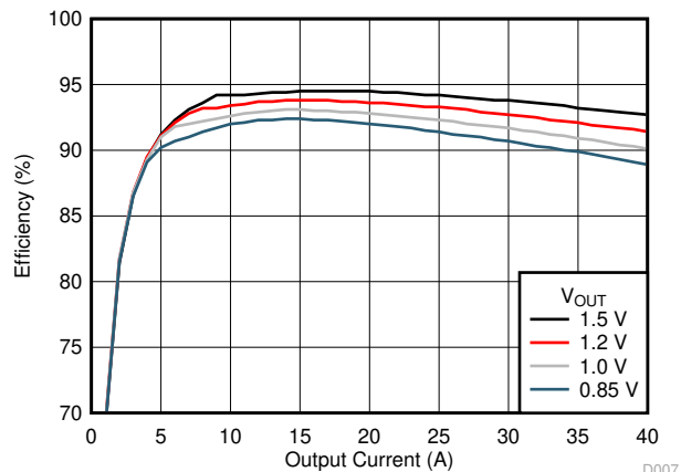
6-2. VOUTB Efficiency
