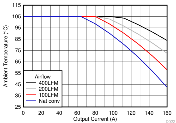
ⓧ 6-8. Thermal Safe Operating Area
