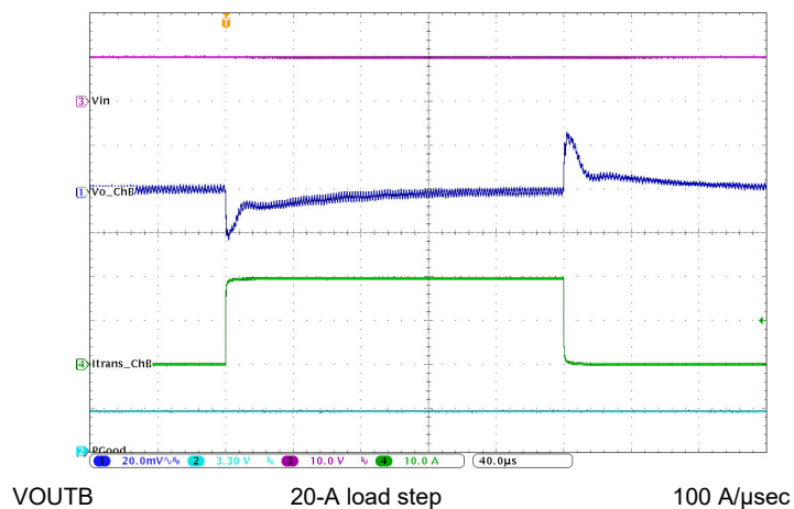
8-14. Transient Response
