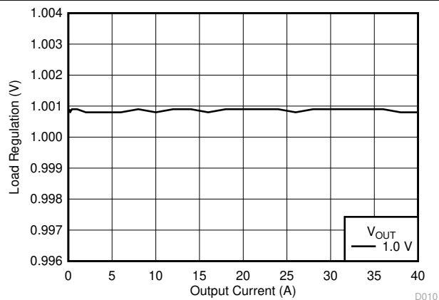
6-6. VOUTB Load Regulation
