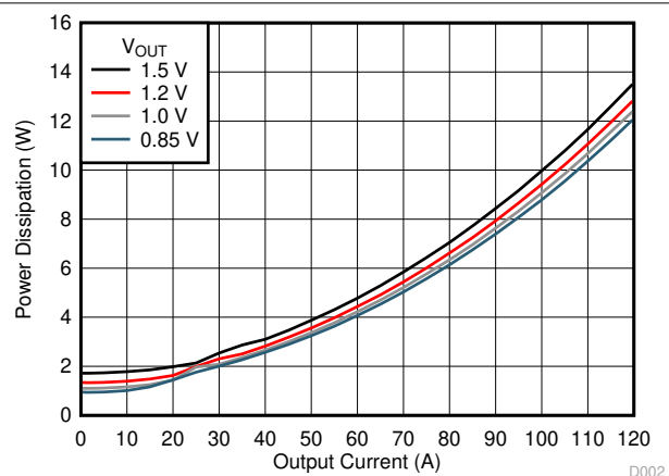
6-3. VOUTA Power Dissipation
