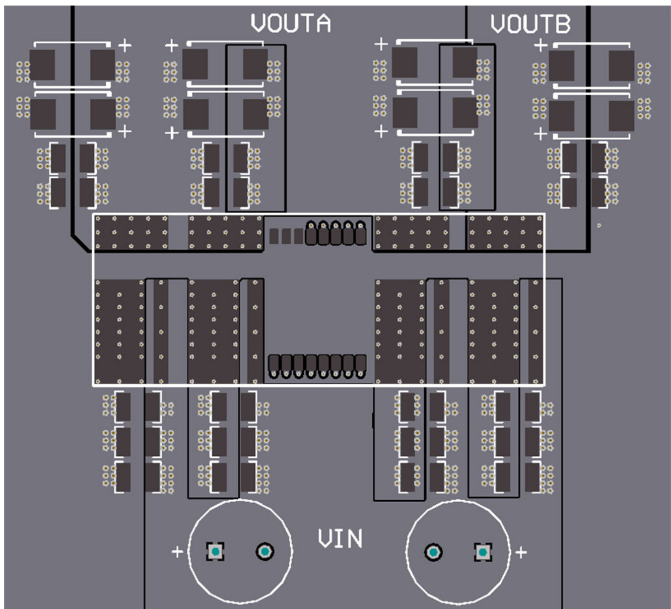
✎ 10-1. Top Layer (Top View)
