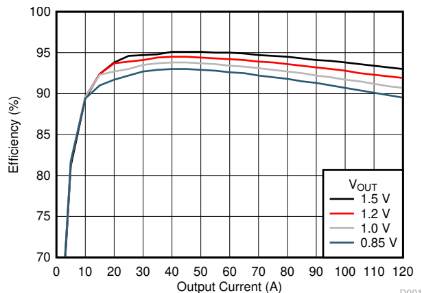
6-1. VOUTA Efficiency
