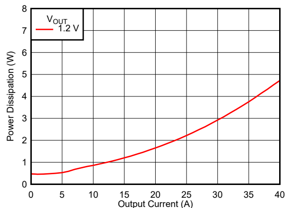
8-5. VOUTB Power Dissipation
