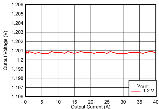
8-7. VOUTB Load Regulation
