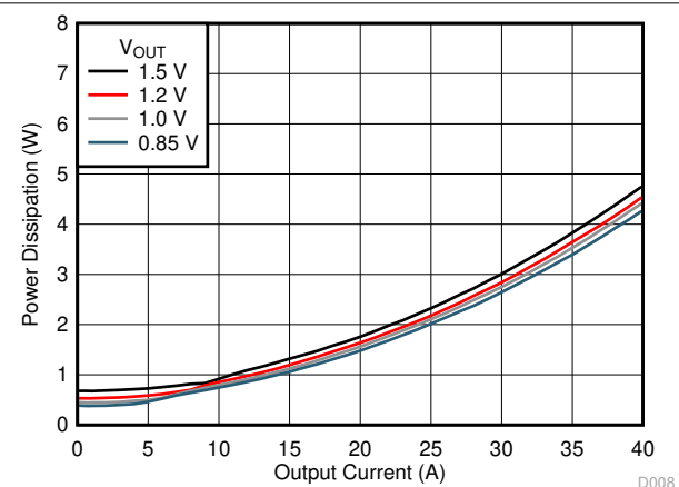
6-4. VOUTB Power Dissipation
