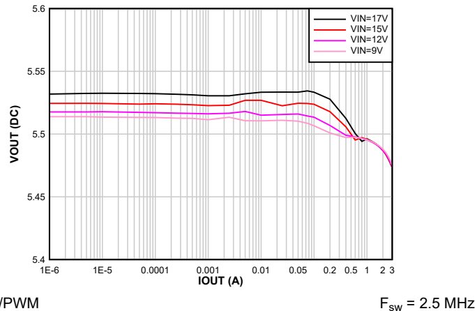
FIG 8-60. Output Voltage vs Output Current V_{OUT} = 5.5\text{ V}
