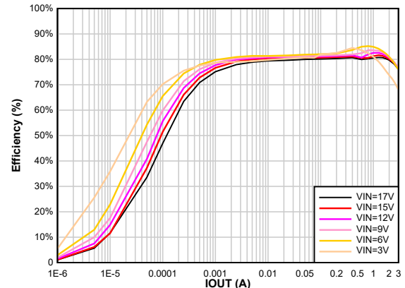
8-6. Efficiency vs Output Current V_{OUT} = 1.2 \text{ V}
