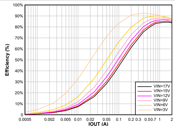
8-8. Efficiency vs Output Current V_{OUT} = 1.8 \text{ V}
