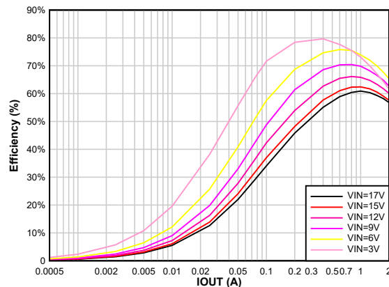
8-55. Efficiency vs Output Current V_{OUT} = 0.4 \text{ V}
