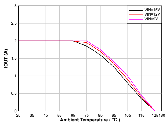
8-46. Thermal Derating V_{OUT} = 3.3\text{ V}
