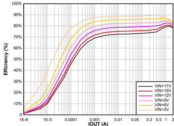
8-5. Efficiency vs Output Current V_{OUT} = 1.2 \text{ V}
