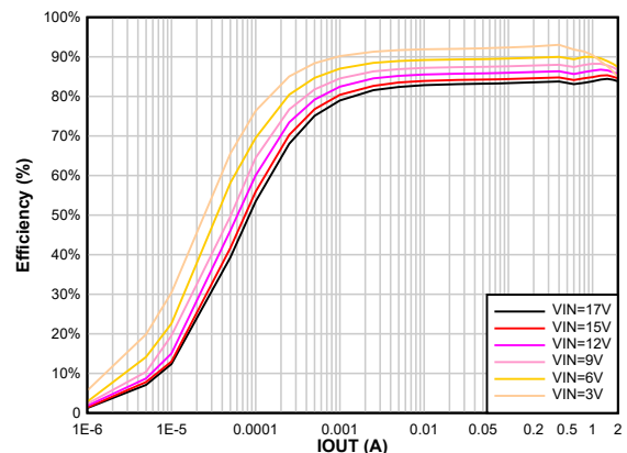
8-6. Efficiency vs Output Current V_{OUT} = 1.2 \text{ V}
