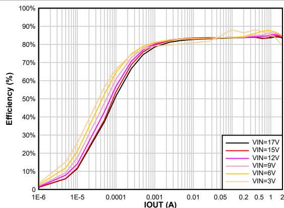
8-7. Efficiency vs Output Current V_{OUT} = 1.2 \text{ V}
