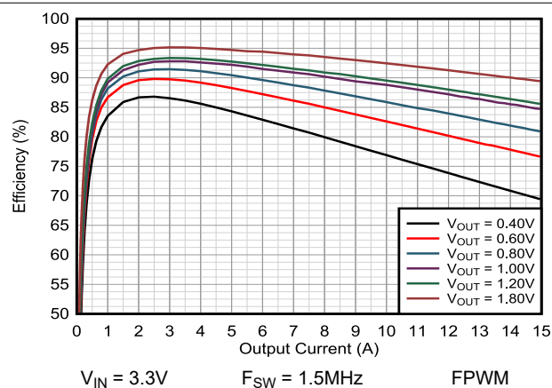
9-10. Efficiency TPSM8287A15BAM
