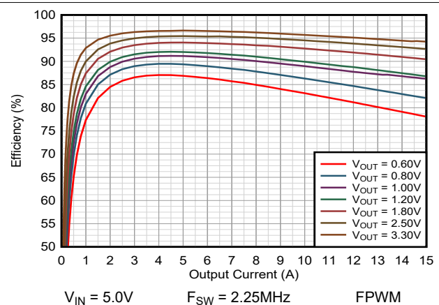
9-13. Efficiency TPSM8287A15BBM
