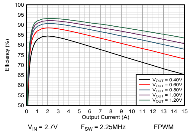
9-9. Efficiency TPSM8287A15BBM
