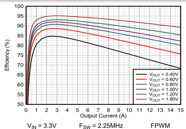
9-11. Efficiency TPSM8287A15BBM
