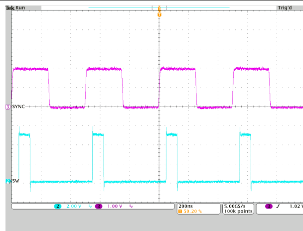
図 9-25. Synchronization to an External Clock
