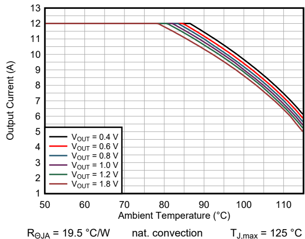
9-42. Safe Operating Area TPSM8287A12BAS V_{IN} = 3.3\text{ V}
