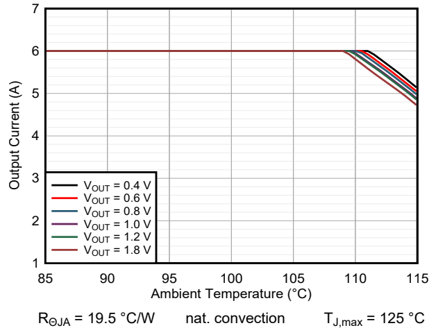
9-38. Safe Operating Area TPSM8287A06BAS V_{IN} = 3.3\text{ V}
