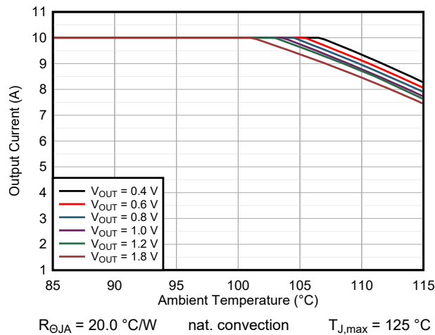
9-40. Safe Operating Area TPSM8287A10BAH V_{IN} = 3.3\text{ V}
