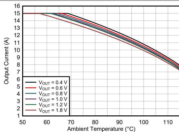
図 9-48. Safe Operating Area TPSM8287A15BBH V_{IN} = 3.3\text{ V}
