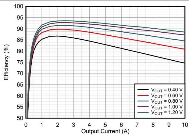
図 9-3. Efficiency TPSM8287A10BAH
