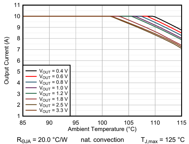
9-41. Safe Operating Area TPSM8287A10BAH V_{IN} = 5.0\text{ V}
