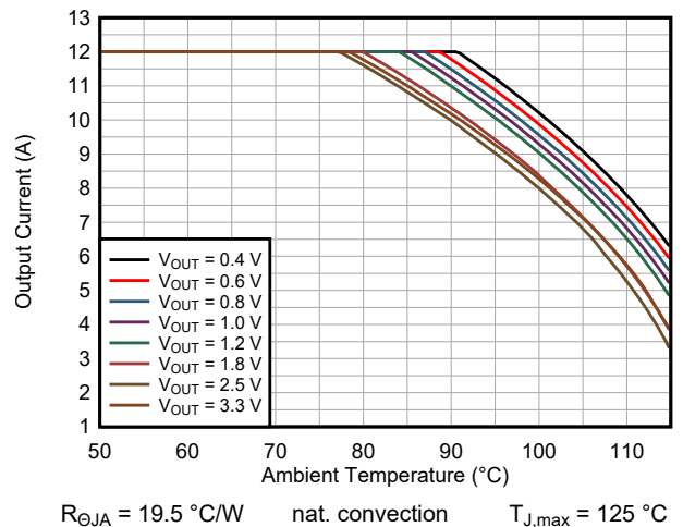
9-43. Safe Operating Area TPSM8287A12BAS V_{IN} = 5.0\text{ V}
