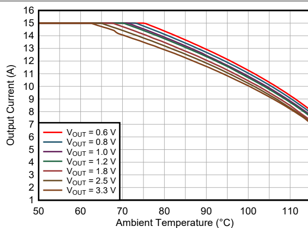
図 9-49. Safe Operating Area TPSM8287A15BBH V_{IN} = 5.0\text{ V}
