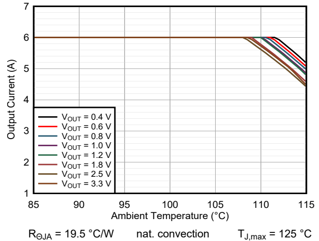
9-39. Safe Operating Area TPSM8287A06BAS V_{IN} = 5.0\text{ V}
