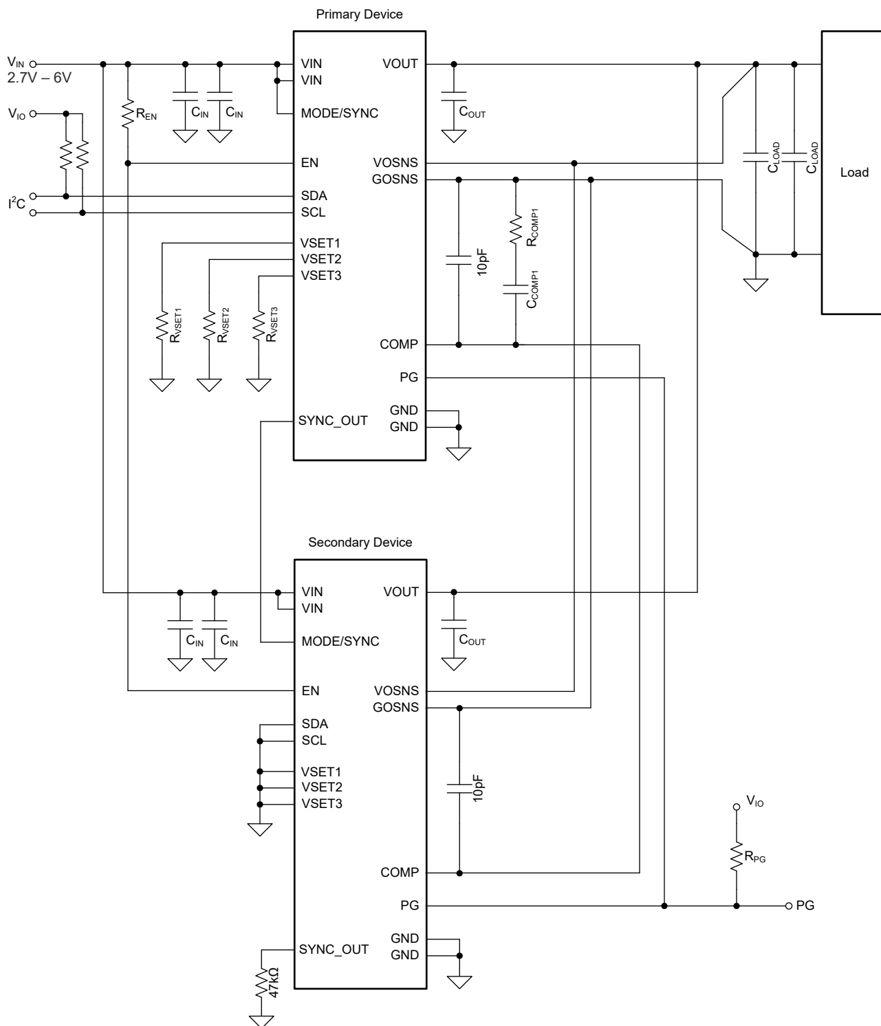
7-21. Two TPSM8287A1xM Devices in a Stacked Configuration
