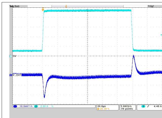
図 9-26. Load Transient Response TPSM8287A12BBS
