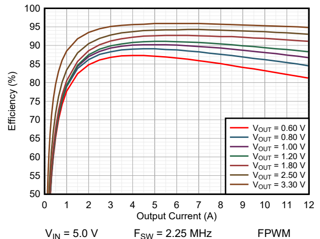
図 9-13. Efficiency TPSM8287A12BBS
