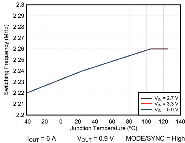
Figure 6-3. TPSM8287A12BBS Switching Frequency vs T_J
