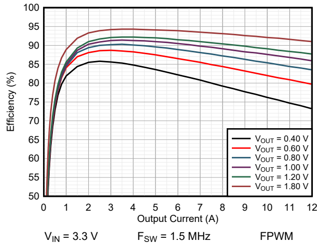
図 9-10. Efficiency TPSM8287A12BAS
