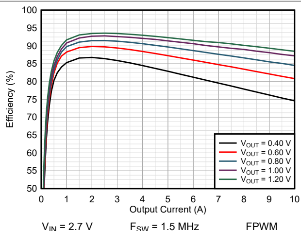
図 9-3. Efficiency TPSM8287A10BAH
