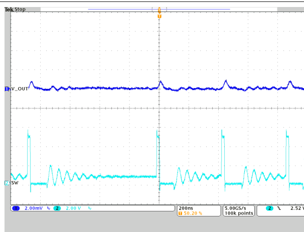
図 9-29. PFM-DCM Operation TPSM8287A12BBS
