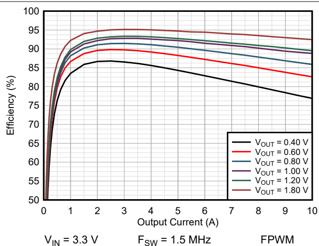
図 9-5. Efficiency TPSM8287A10BAH
