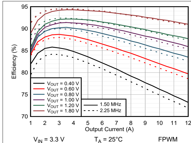
図 7-14. Efficiency Comparison TPSM8287A12BAS vs TPSM8287A12BBS
