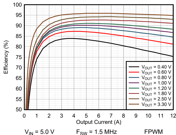
図 9-12. Efficiency TPSM8287A12BAS
