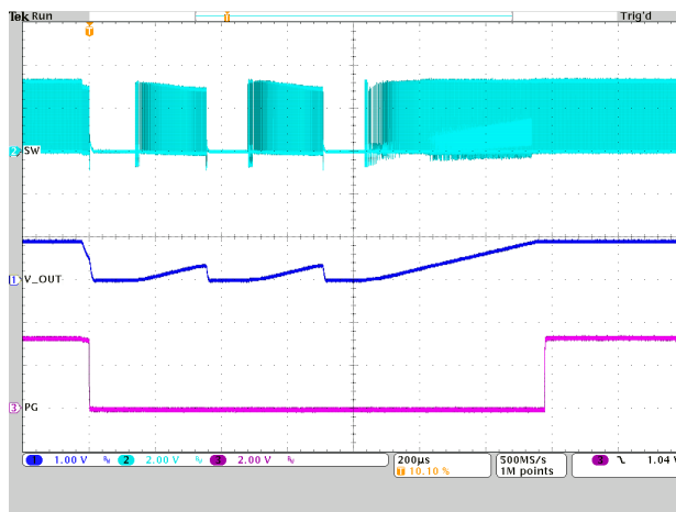
FIG 7-19. Hiccup Current Limit
