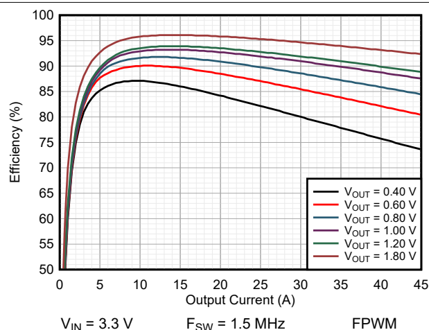
図 9-53. Efficiency
