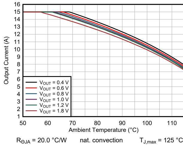
図 9-48. Safe Operating Area TPSM8287A15BBH V_{IN} = 3.3\text{ V}
