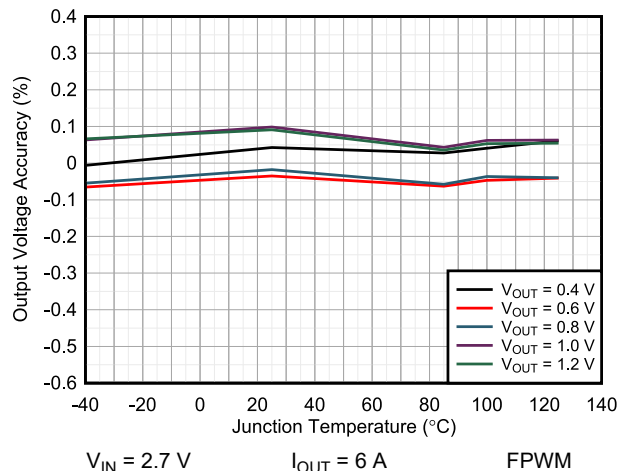
9-21. Vout Accuracy vs Temperature TPSM8287A12BAS
