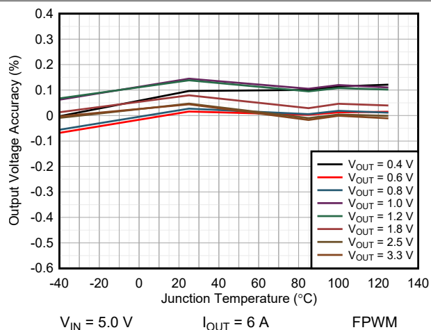
9-25. Vout Accuracy vs Temperature TPSM8287A12BAS
