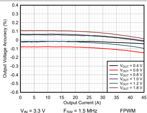
図 9-54. Load Regulation
