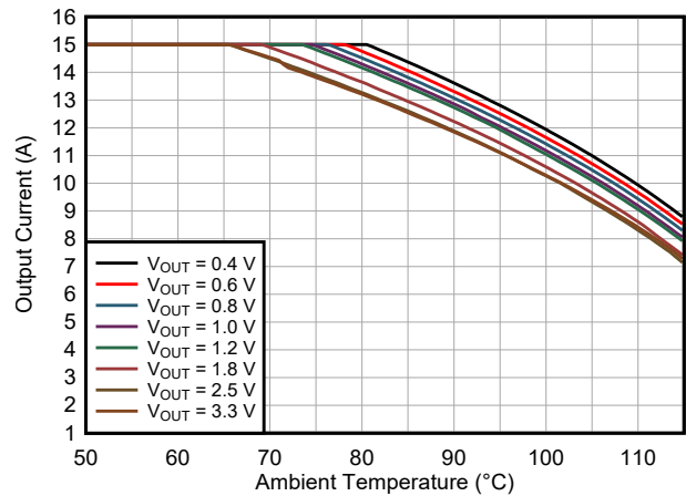
図 9-45. Safe Operating Area TPSM8287A12BBS V_{IN} = 5.0\text{ V}
