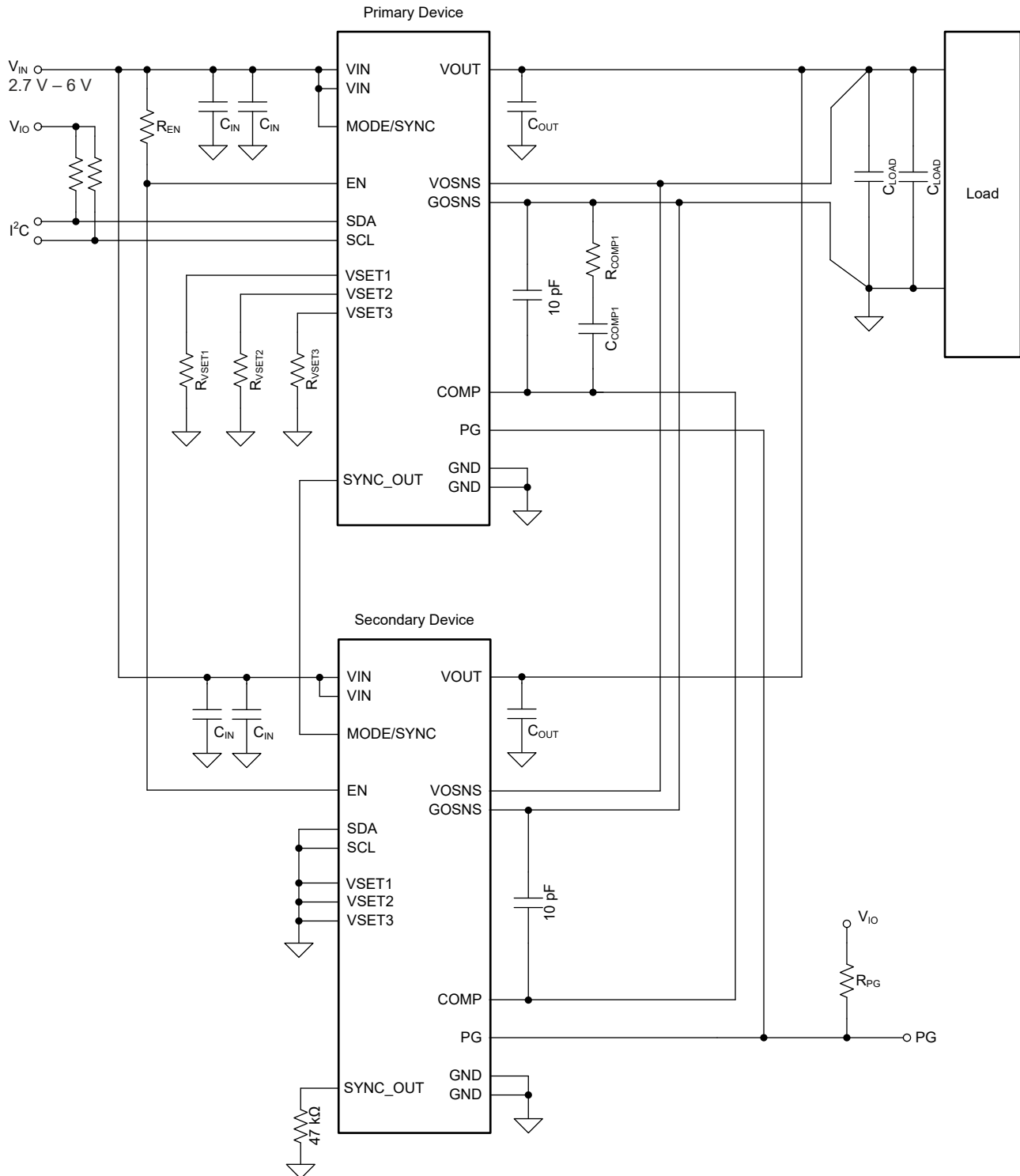
☒ 7-22. Two TPSM8287Axx Devices in a Stacked Configuration
