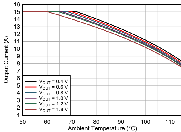
図 9-44. Safe Operating Area TPSM8287A12BBS V_{IN} = 3.3\text{ V}
