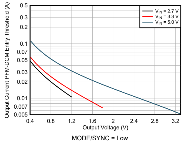
図 7-8. PFM-DCM Entry Threshold TPSM8287A10BAH, TPSM8287A15BAH
