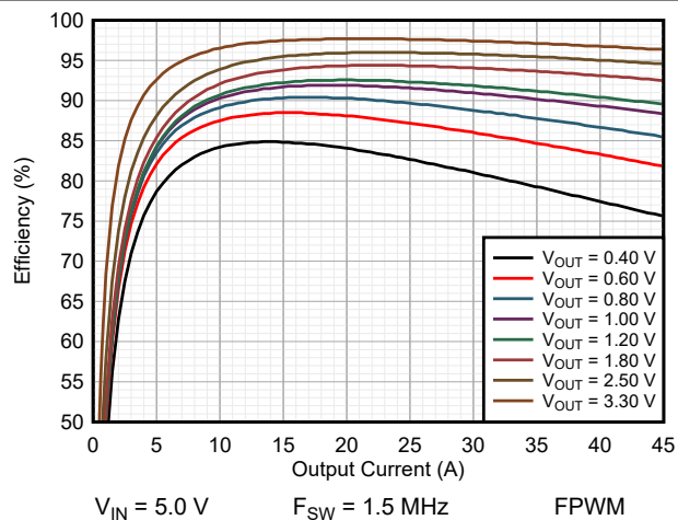
9-55. Efficiency
