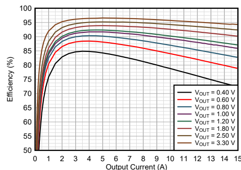
効率性 TPSM8287A15BAH ( V_{IN} = 5.0\text{V} , FPWM)
