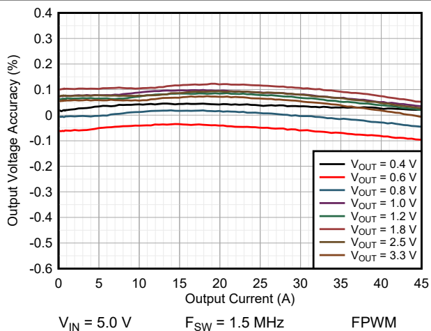
9-56. Load Regulation
