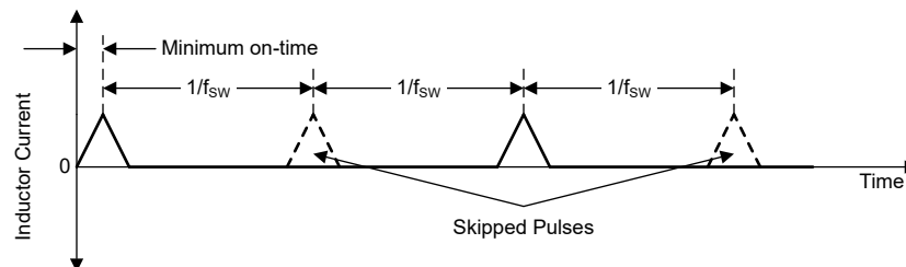
図 7-4. Discontinuous Conduction Mode (PFM-DCM) Current Waveform
