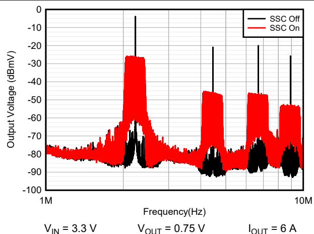
図 9-30. Output Noise over Frequency TPSM8287A12BBS
