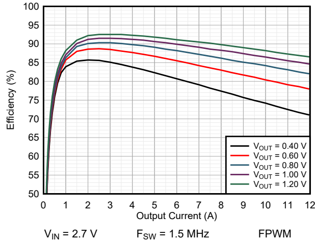
図 9-8. Efficiency TPSM8287A12BAS
