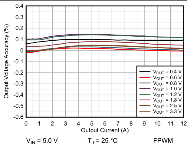
9-24. Load Regulation TPSM8287A12BAS
