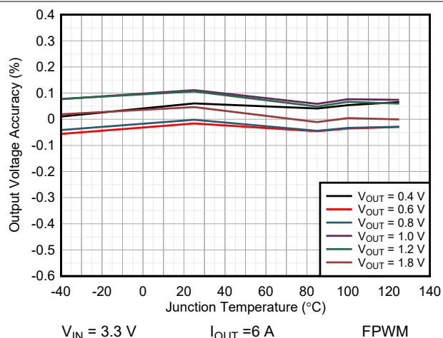
9-23. Vout Accuracy vs Temperature TPSM8287A12BAS
