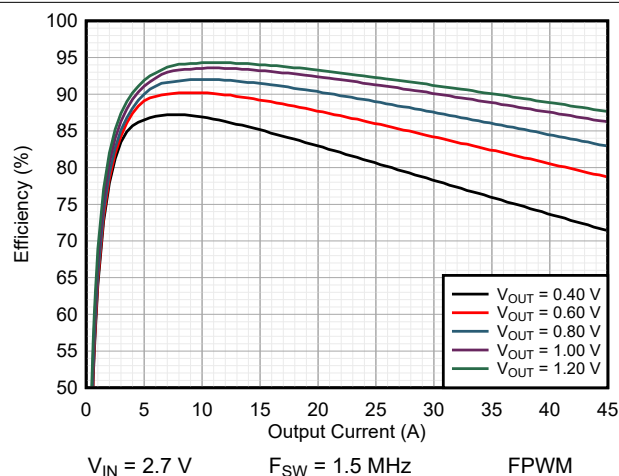
図 9-51. Efficiency
