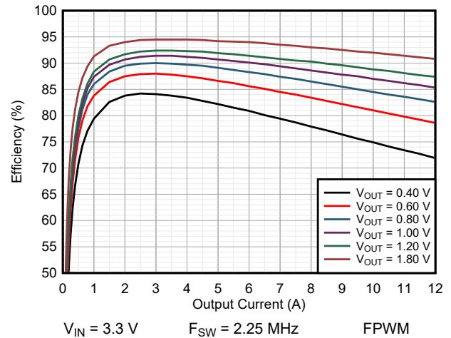
図 9-11. Efficiency TPSM8287A12BBS
