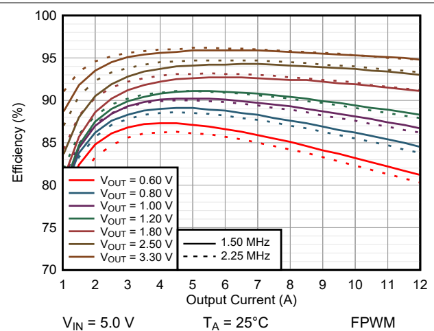
図 7-15. Efficiency Comparison TPSM8287A12BAS vs TPSM8287A12BBS
