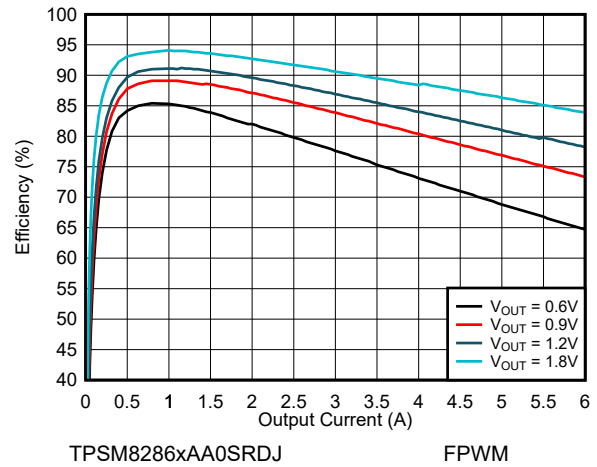
図 8-13. Efficiency V_{IN} = 2.8\text{ V} and T_A = 85^\circ\text{C}
