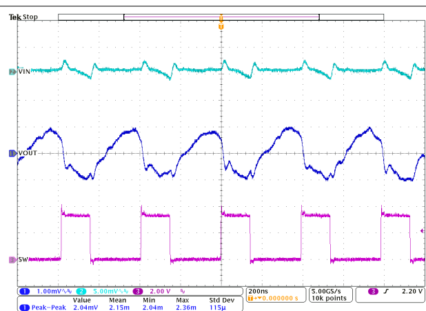
図 8-31. FPWM Operation I_{OUT} = 0.1 \text{ A}
