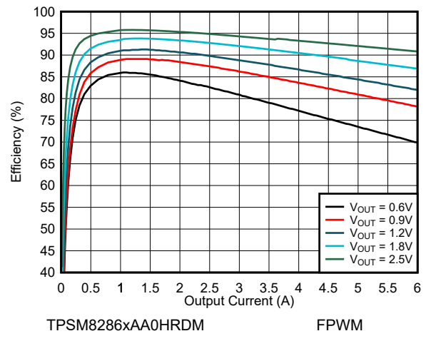
図 8-17. Efficiency V_{IN} = 3.3\text{ V} and T_A = 85^\circ\text{C}
