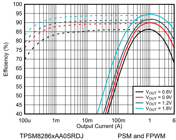
図 8-12. Efficiency V_{IN} = 2.8\text{ V} and T_A = 25^\circ\text{C}
