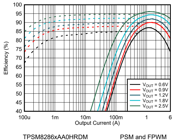
図 8-16. Efficiency V_{IN} = 3.3\text{ V} and T_A = 25^\circ\text{C}
