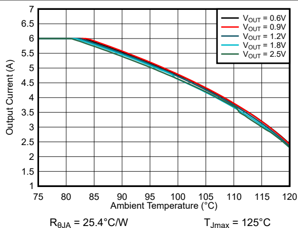
8-40. Safe Operating Area V_{IN} = 3.3\text{-V} TPSM82866AA0SRDJR
