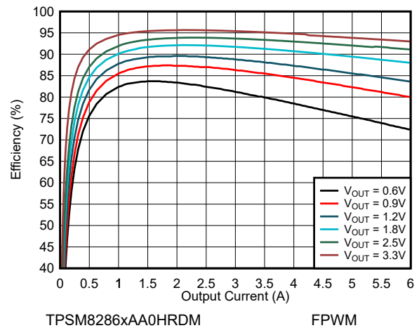
図 8-15. Efficiency V_{IN} = 5.0\text{ V} and T_A = 85^\circ\text{C}
