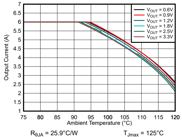
8-43. Safe Operating Area V_{IN} = 5.0\text{-V} TPSM82866AA0HRDMR
