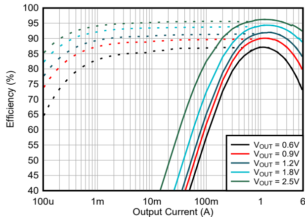
図 8-2. Efficiency V_{IN} = 5.0\text{ V} and T_A = 25^\circ\text{C}
