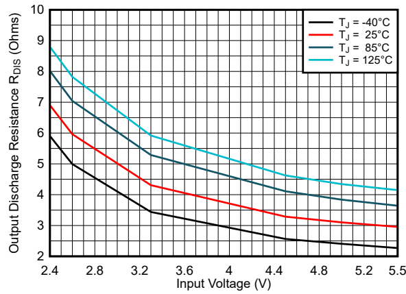
Figure 6-3. Output Discharge Resistance R_{OIS}
