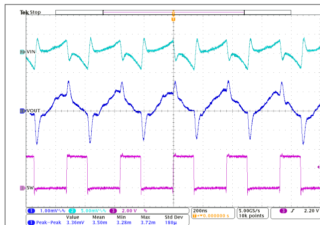
図 8-30. FPWM Operation I_{OUT} = 3 \text{ A}
