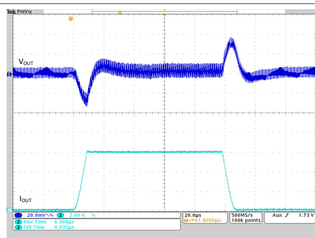
図 8-30. FPWM Operation I_{OUT} = 3 \text{ A}
