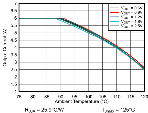
8-42. Safe Operating Area V_{IN} = 3.3\text{-V} TPSM82866AA0HRDMR
