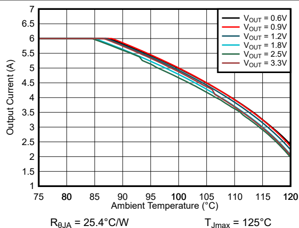
8-41. Safe Operating Area V_{IN} = 5.0\text{-V} TPSM82866AA0SRDJR
