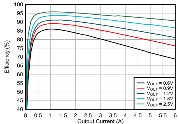
図 8-3. Efficiency V_{IN} = 5.0\text{ V} and T_A = 85^\circ\text{C}
