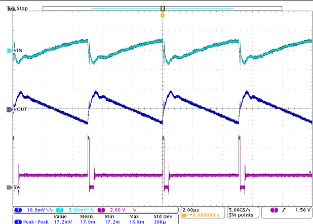
8-27. Switching Frequency V_{IN} = 3.3\text{ V}
