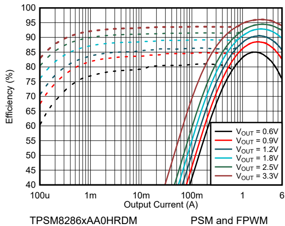
図 8-14. Efficiency V_{IN} = 5.0\text{ V} and T_A = 25^\circ\text{C}
