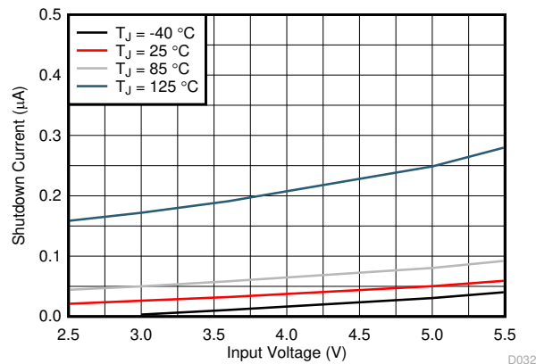
7-5. Shutdown Current
