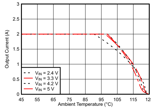
V_{OUT} = 1.2\text{ V} TPSM82822A R_{\theta JA} = 64.3^\circ\text{C/W}
