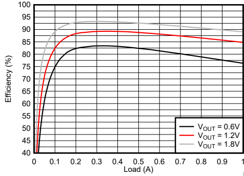
V_{IN} = 2.4\text{ V} T_A = 25^\circ\text{C} TPSM82822A
