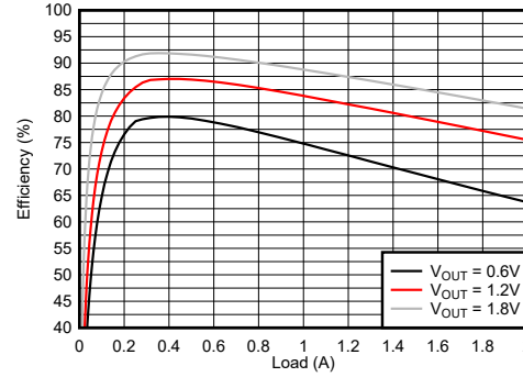
V_{IN} = 2.4\text{ V} T_A = 85^\circ\text{C} TPSM82822A
