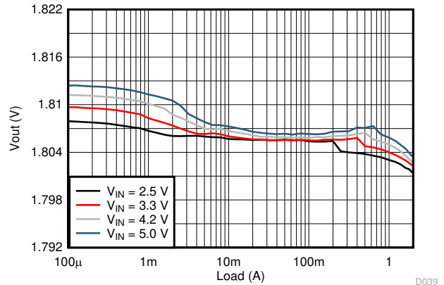
9-66. Load Regulation
