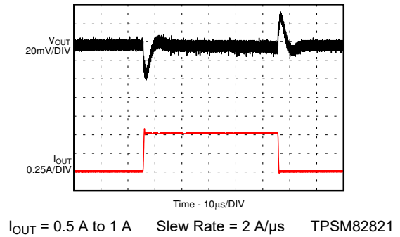
9-26. Load Transient
