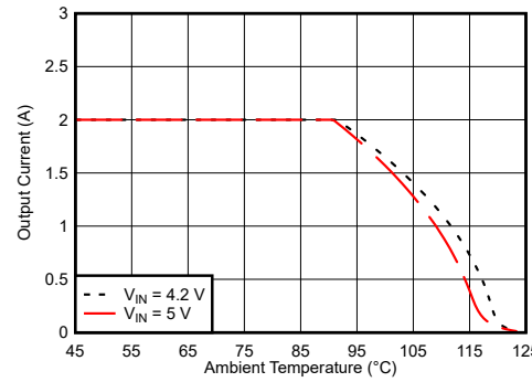
V_{OUT} = 2.5\text{ V} TPSM82822A R_{\theta JA} = 64.3^\circ\text{C/W}
