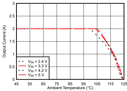
V_{OUT} = 0.6\text{ V} TPSM82822A R_{\theta JA} = 64.3^\circ\text{C/W}
