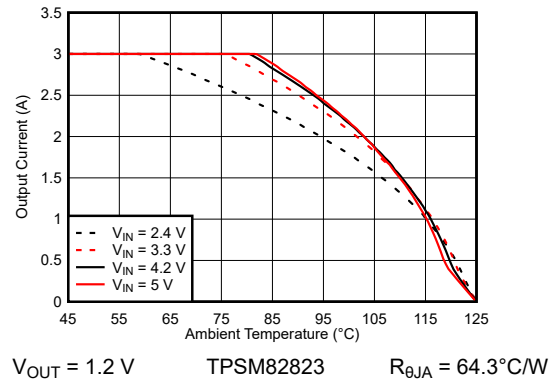
9-119. Safe Operating Area
