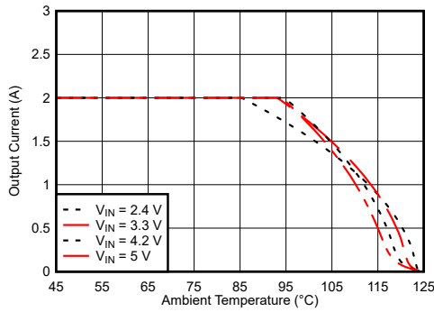
V_{OUT} = 1.8\text{ V} TPSM82822A R_{\theta JA} = 64.3^\circ\text{C/W}
