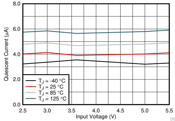
7-4. Quiescent Current
