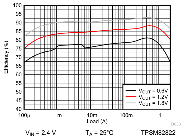
9-59. Efficiency
