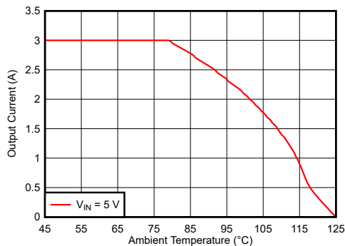
FIG 9-122. Safe Operating Area
