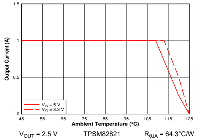
Figure 9-14. Safe Operating Area
