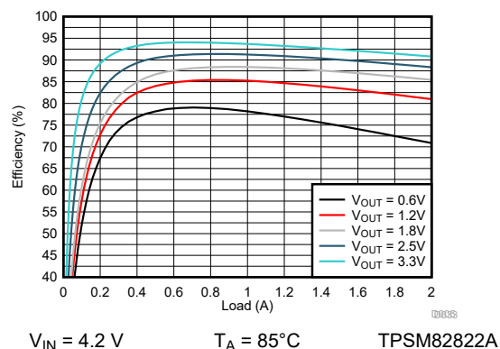
Figure 9-89. Efficiency
