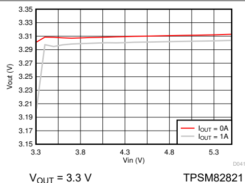
9-24. Line Regulation
