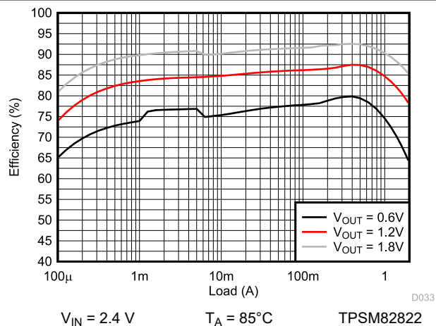
9-60. Efficiency
