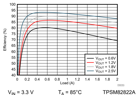
Figure 9-91. Efficiency
