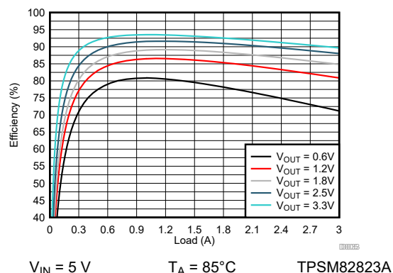
图 9-138. Efficiency
