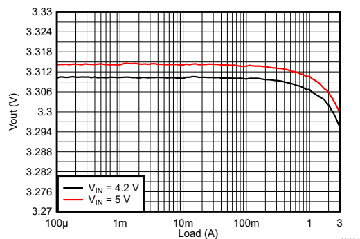
9-152. Load Regulation
