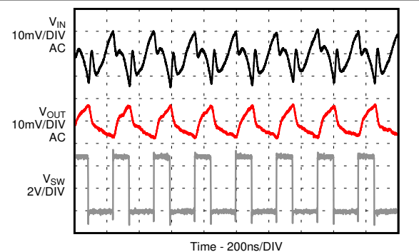
9-76. Input and Output Ripple in PWM Mode
