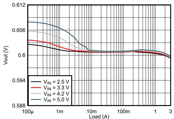
FIG 9-123. Load Regulation
