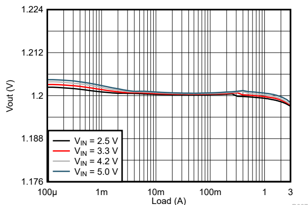
FIG 9-124. Load Regulation
