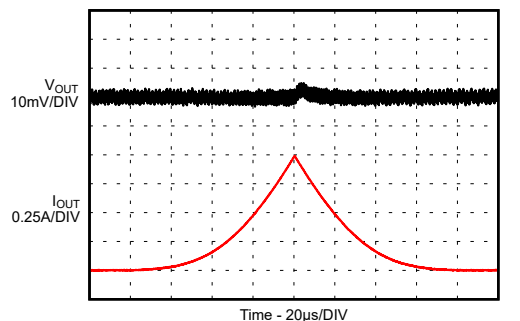
9-48. Load Sweep
