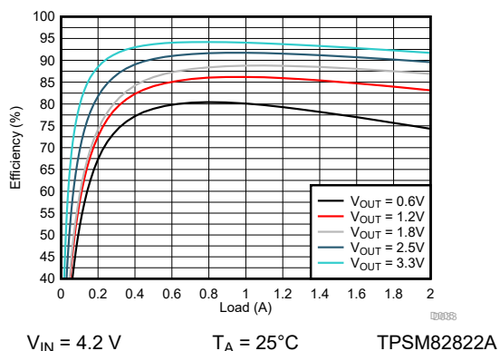
Figure 9-88. Efficiency
