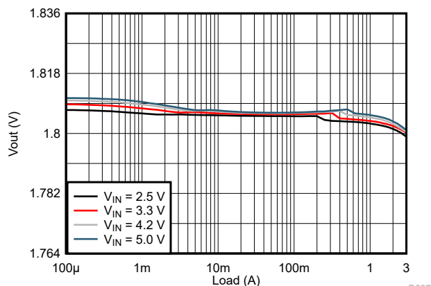
FIG 9-123. Load Regulation
