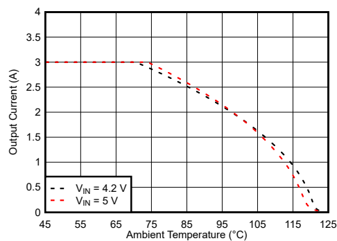
图 9-148. Safe Operating Area
