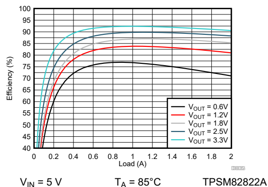
Figure 9-87. Efficiency
