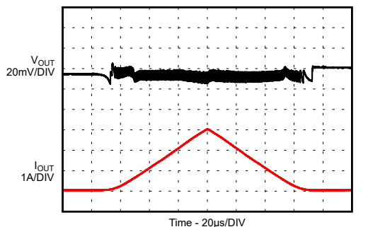
9-130. Load Sweep
