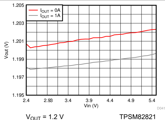
9-22. Line Regulation
