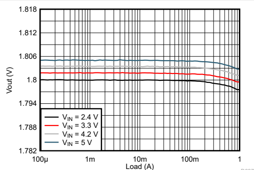
9-42. Load Regulation
