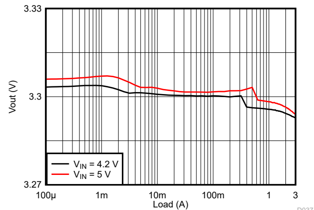
FIG 9-125. Load Regulation
