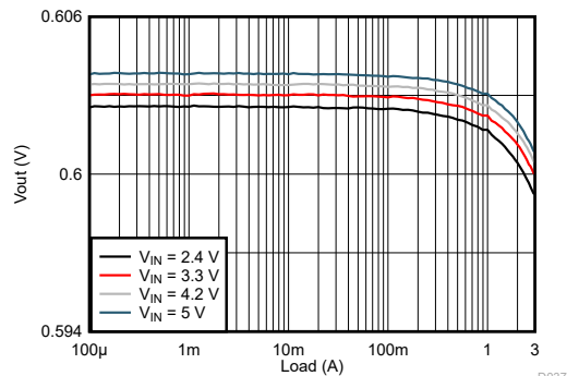
9-150. Load Regulation
