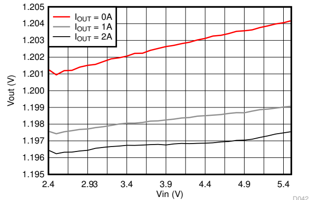
9-72. Line Regulation
