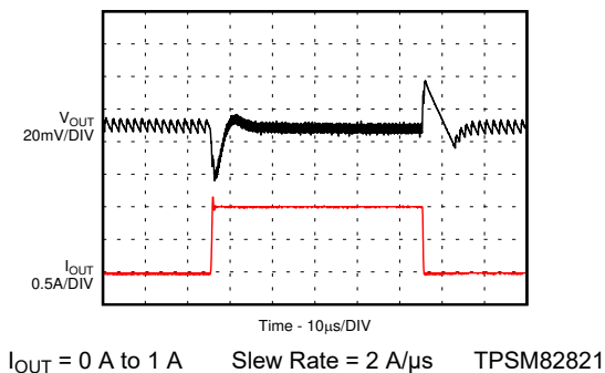
9-25. Load Transient
