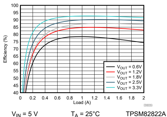
Figure 9-86. Efficiency
