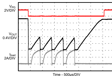
9-135. Short Circuit, HICUP Protection Entry / Exit
