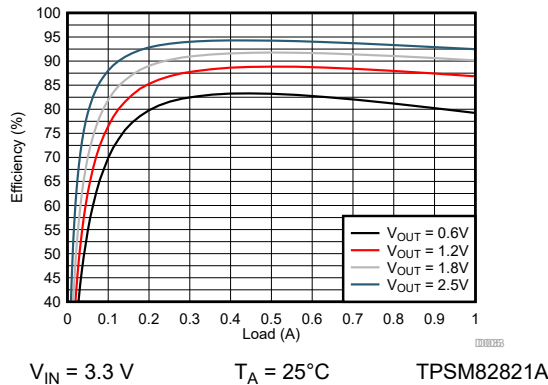
Figure 9-33. Efficiency
