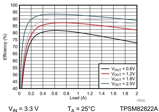
Figure 9-90. Efficiency
