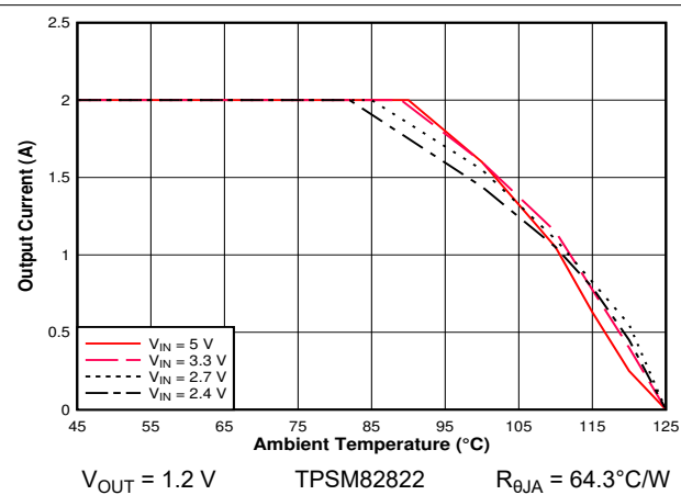
9-62. Safe Operating Area
