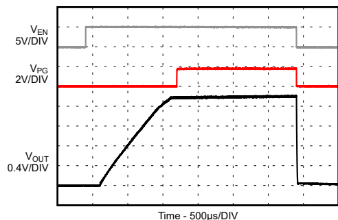
9-134. Start-up / Shutdown with Resistive Load
