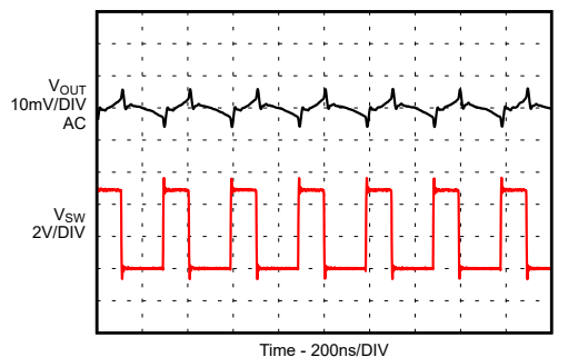
9-47. Output Ripple in PWM Mode
