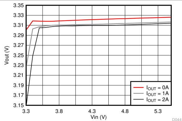
9-73. Line Regulation
