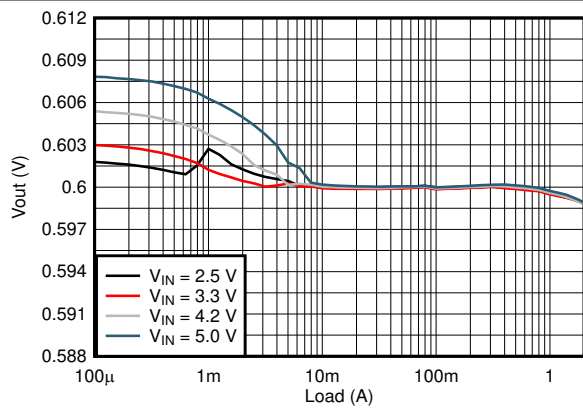
9-66. Load Regulation
