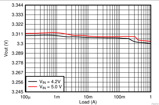
9-18. Load Regulation
