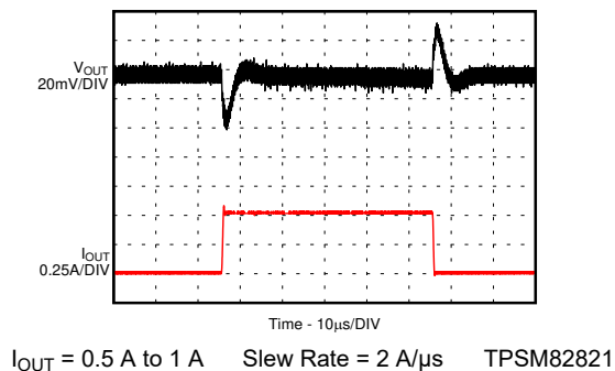
9-26. Load Transient
