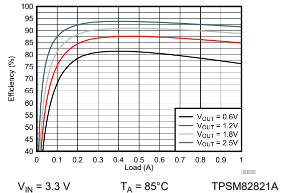
Figure 9-34. Efficiency
