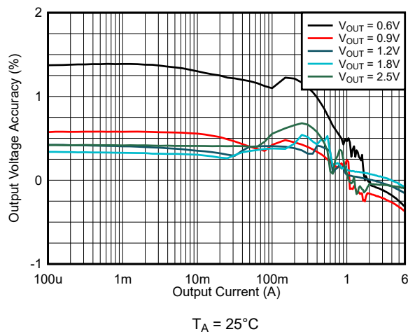
8-16. Load Regulation V_{IN} = 3.3\text{ V} (PSM)
