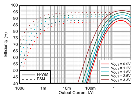
TPSM82816PVCA の効率 ( V_{IN} = 5V )
