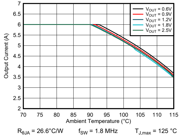
8-21. TPSM82816PVCA Safe Operating Area V_{\text{IN}} = 3.3 \text{ V}
