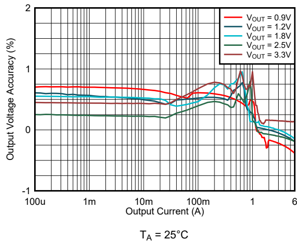
8-14. Load Regulation V_{IN} = 5.0\text{ V} (PSM)
