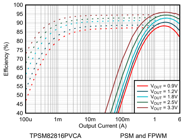
8-2. Efficiency V_{IN} = 5.0\text{ V} and T_A = 25^\circ\text{C}
