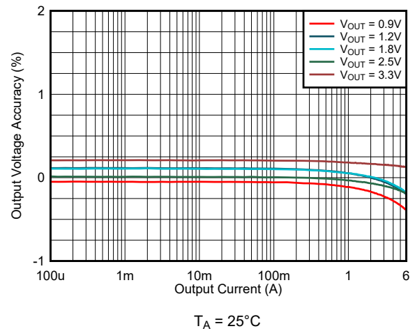
8-15. Load Regulation V_{IN} = 5.0\text{ V} (FPWM)
