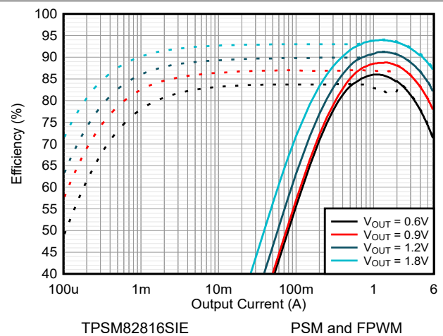
8-7. Efficiency V_{IN} = 2.7\text{ V} and T_A = 25^\circ\text{C}
