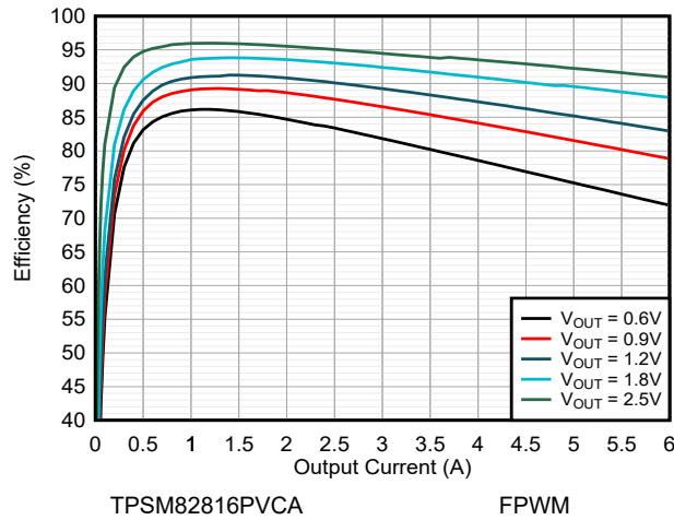
8-10. Efficiency V_{IN} = 3.3\text{ V} and T_A = 85^\circ\text{C}
