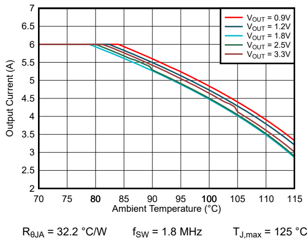
8-22. TPSM82816SIE Safe Operating Area V_{\text{IN}} = 5.0 \text{ V}
