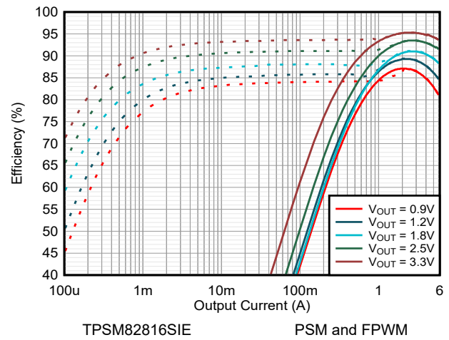
8-3. Efficiency V_{IN} = 5.0\text{ V} and T_A = 25^\circ\text{C}
