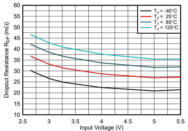
図 6-6. Dropout Resistance TPSM82816SIE
