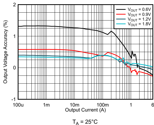
8-18. Load Regulation V_{IN} = 2.7\text{ V} (PSM)
