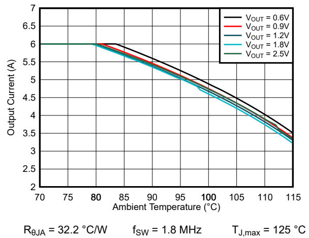
8-23. TPSM82816SIE Safe Operating Area V_{\text{IN}} = 3.3 \text{ V}
