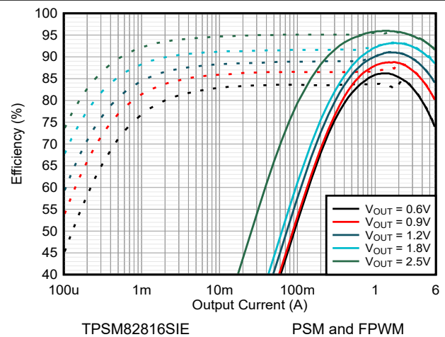
8-5. Efficiency V_{IN} = 3.3\text{ V} and T_A = 25^\circ\text{C}
