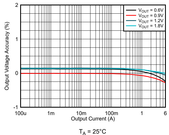
8-19. Load Regulation V_{IN} = 2.7\text{ V} (FPWM)
