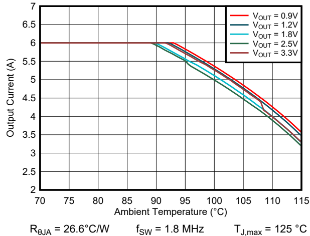
8-20. TPSM82816PVCA Safe Operating Area V_{\text{IN}} = 5.0 \text{ V}
