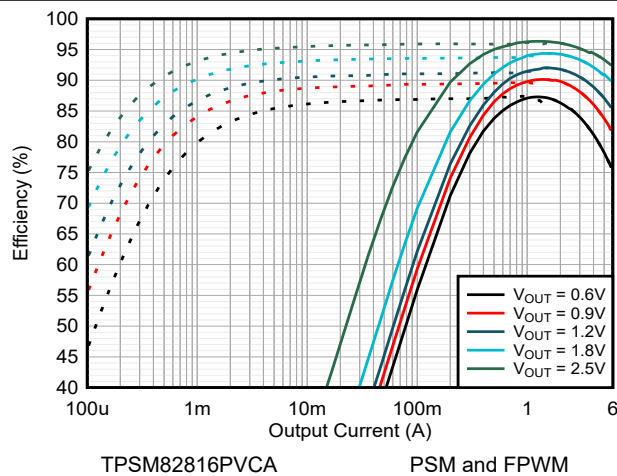
8-4. Efficiency V_{IN} = 3.3\text{ V} and T_A = 25^\circ\text{C}
