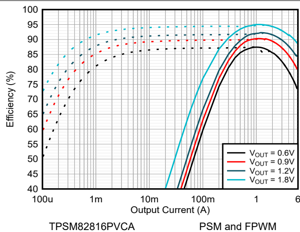
8-6. Efficiency V_{IN} = 2.7\text{ V} and T_A = 25^\circ\text{C}
