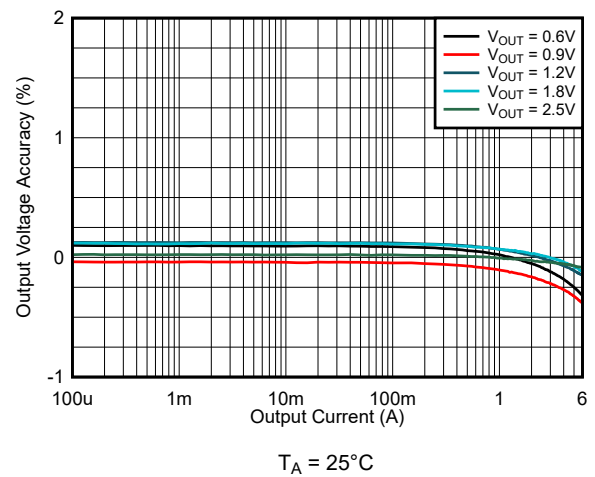
8-17. Load Regulation V_{IN} = 3.3\text{ V} (FPWM)
