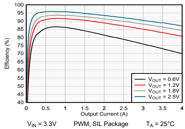
図 9-3. Efficiency vs Output Current
