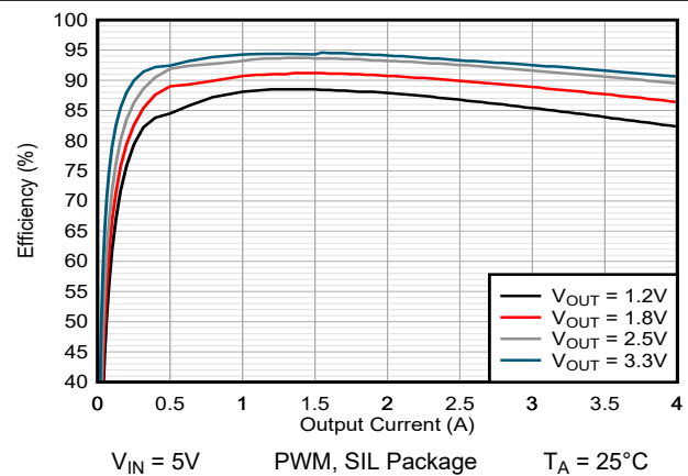
図 9-7. Efficiency vs Output Current
