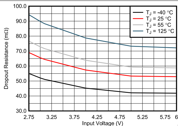
Figure 6-4. Dropout Resistance
