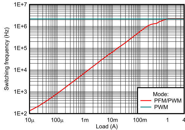
図 8-1. Switching Frequency versus Output Current ( V_{IN} = 5V , V_{OUT} = 1.8V , R_{CF} = 8.06k\Omega )
