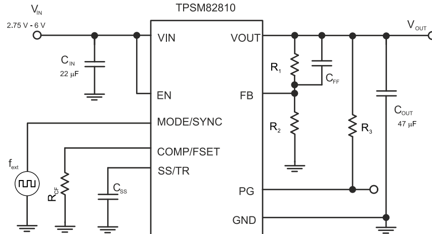
Figure 9-35. Frequency Synchronization
