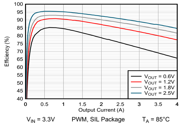
図 9-5. Efficiency vs Output Current
