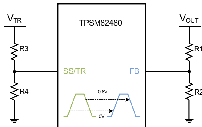
Figure 9. Voltage Tracking
