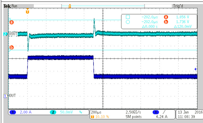
30. Load Transient Response (PSM-PWM), Load Step 0 to 3 A
