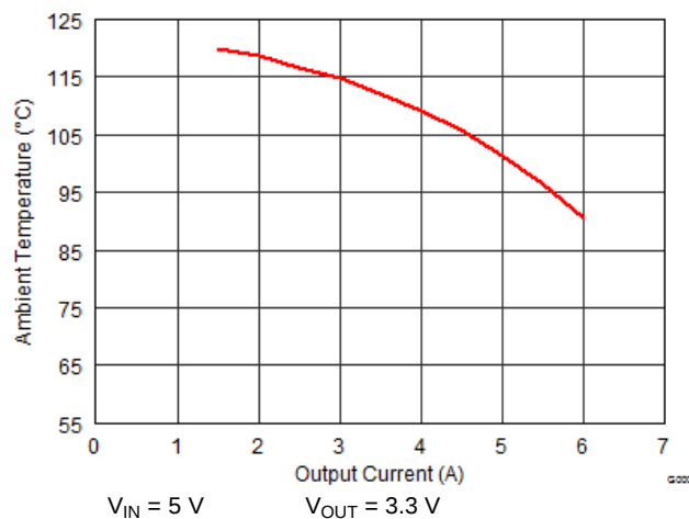
FIG 36. Maximum Ambient Temperature for T_J=125^\circ\text{C} (TPSM82480 EVM)
