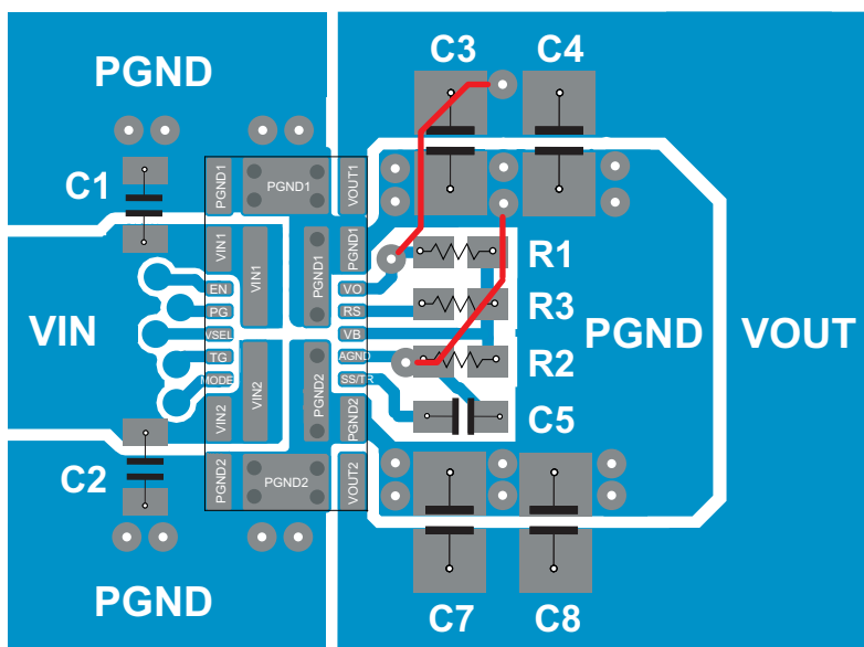
39. TPSM82480 Board Layout
