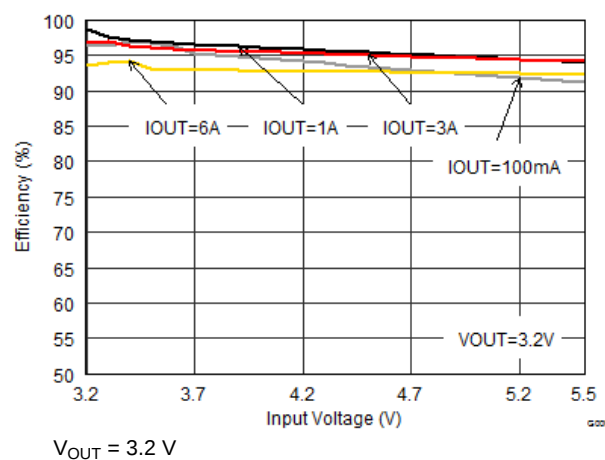
FIG 11. Efficiency vs Input Voltage
