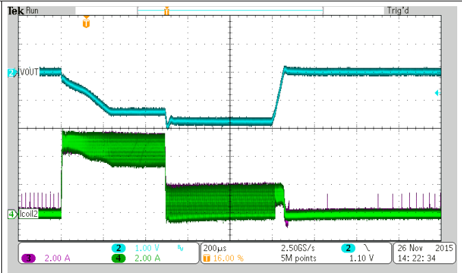
FIG 35. Current Limit Fold-Back at Overload
