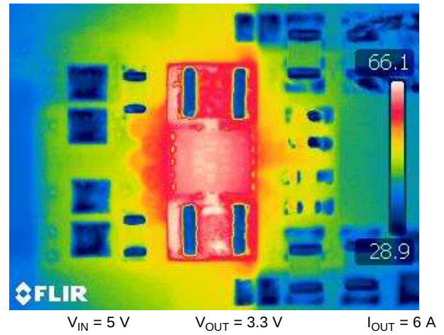
FIG 37. Device Temperature (TPSM82480 EVM)
