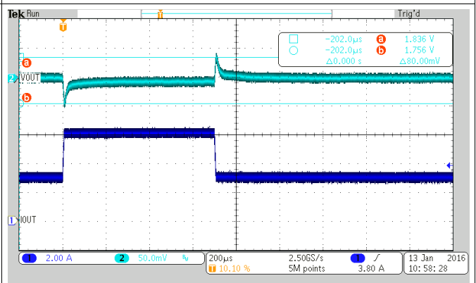
31. Load Transient Response (PSM-PWM), Load Step 0 to 3 A
