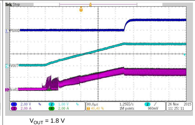
23. Startup into 0.3 Ω resistor
