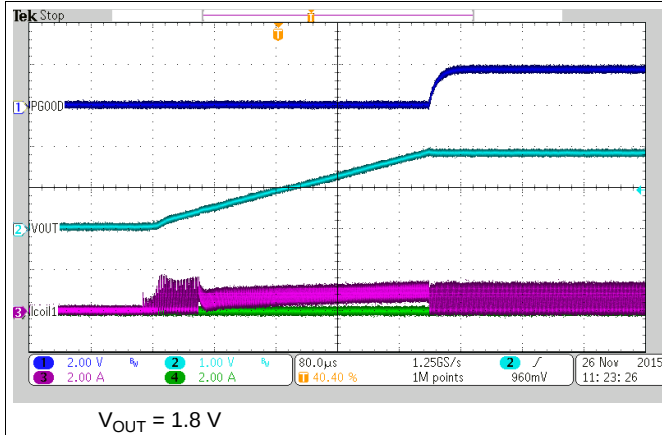
22. Startup into 3.3 Ω resistor
