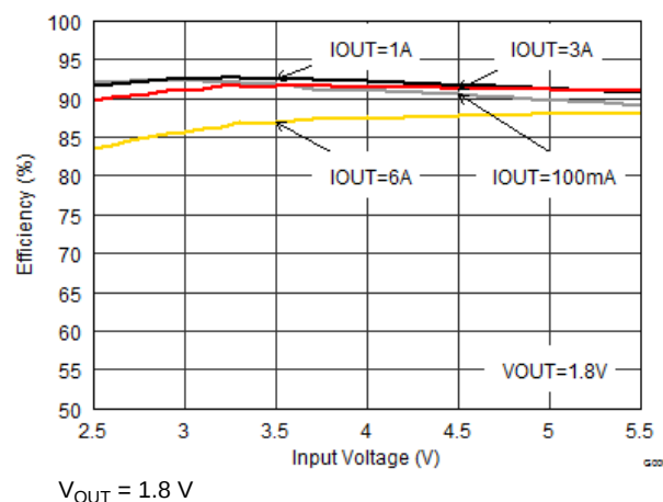
FIG 13. Efficiency vs Input Voltage
