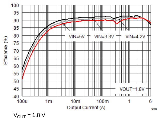
FIG 12. Efficiency vs Output Current
