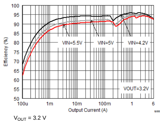
FIG 10. Efficiency vs Output Current
