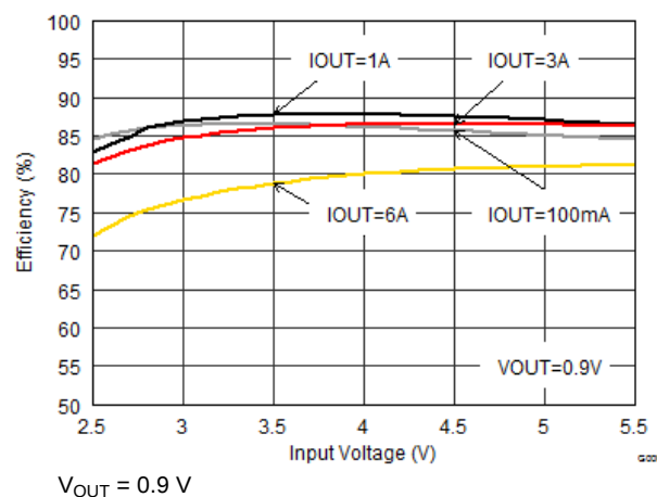
FIG 15. Efficiency vs Input Voltage
