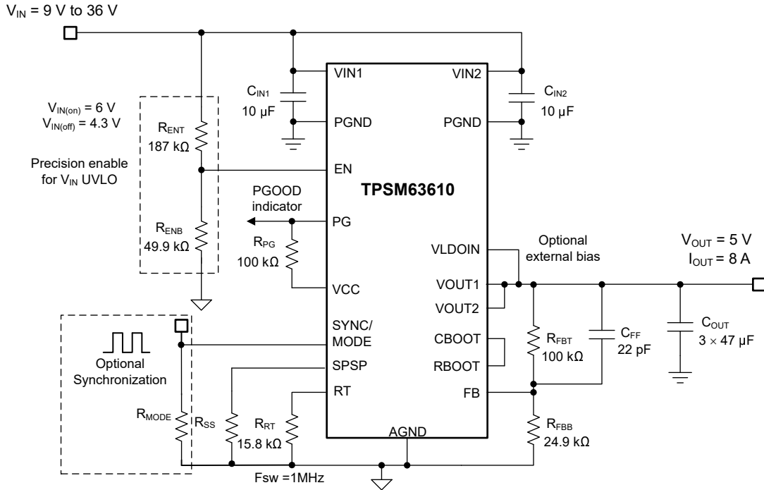
図 8-21. Circuit Schematic
