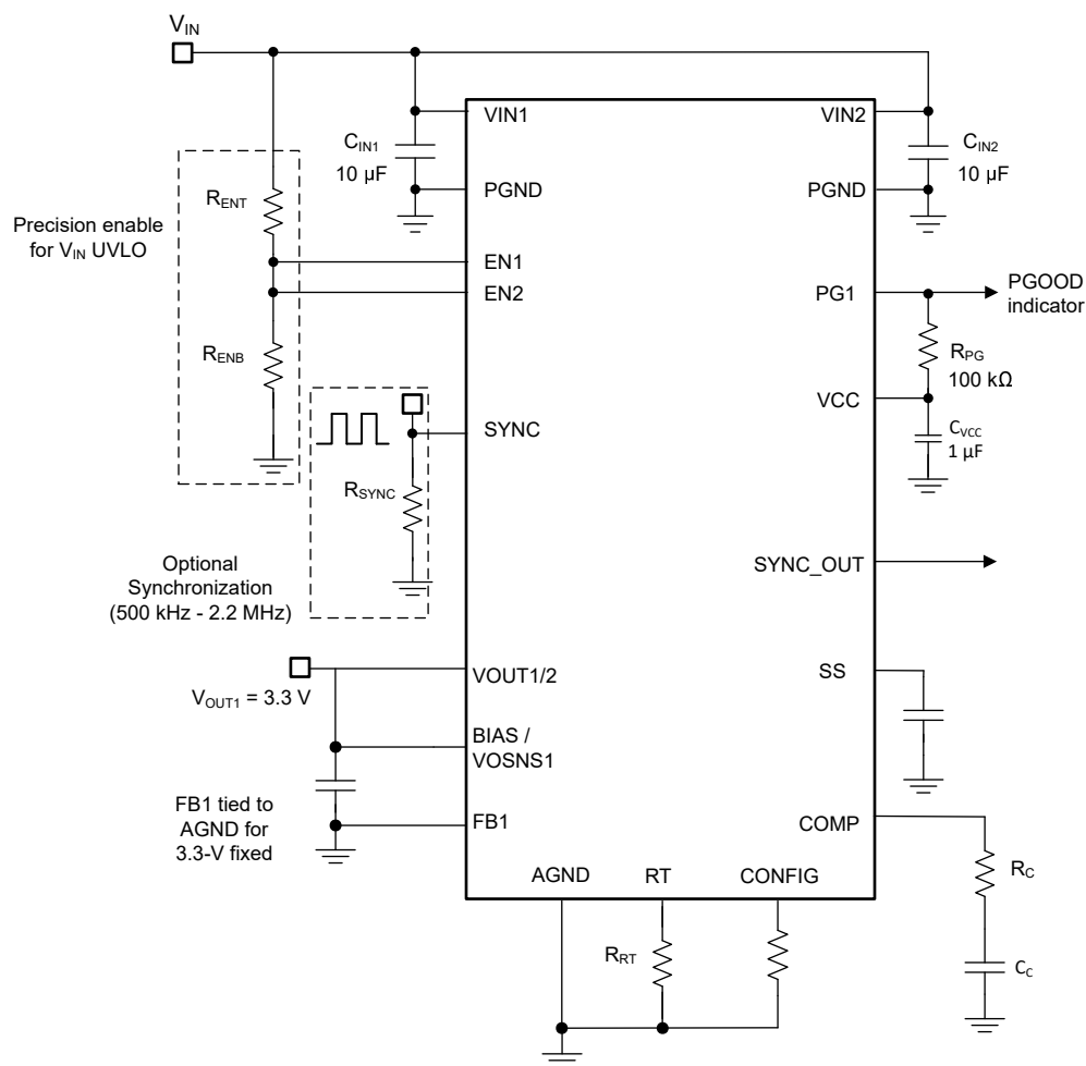
図 7-3. High-efficiency, Single Output 2-Phase Step-down Converter
