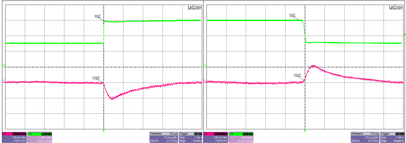
VOUT2 = 3.3 V, IOUT2 = 3 A to 6 A at 1 A/μs 図 8-12. Load Transient Rising (CH2)
