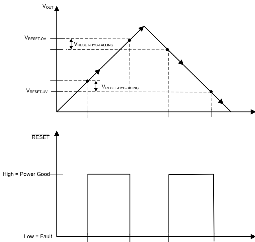
図 7-9. PG Static Voltage Thresholds
