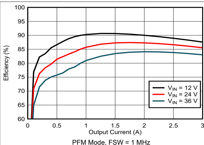
図 8-3. Efficiency, V_{OUT} = 3.3\text{ V}
