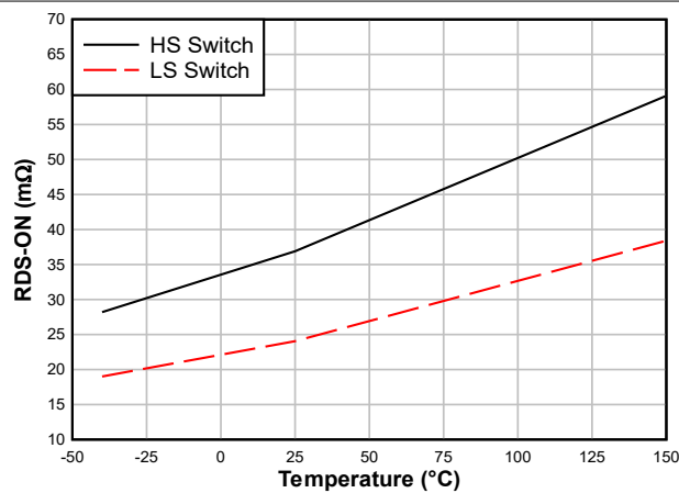
図 6-3. High-side and Low-side Switches R_{DS\_ON}
