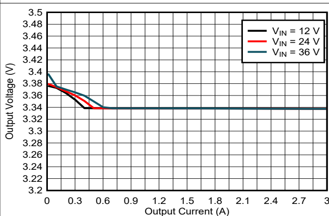
図 8-5. Load Regulation, V_{OUT} = 3.3\text{ V} , PFM Mode
