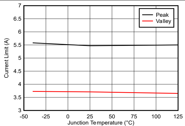
図 6-4. High-side and Low-side Current Limits TPSM64406
