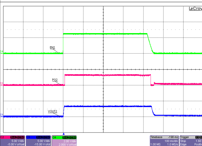
図 8-7. Start-up and Shut-down, VOUT2 = 3.3 V
