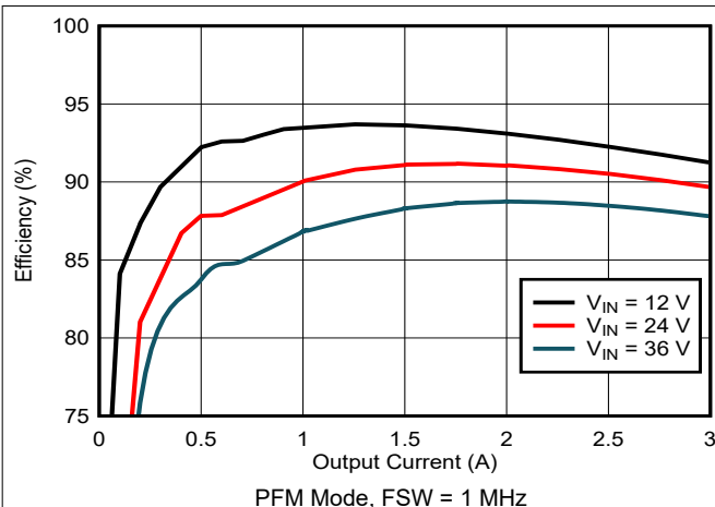
図 8-2. Efficiency, V_{OUT} = 5\text{ V}
