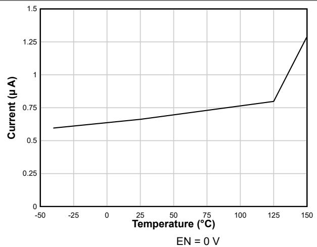
図 6-2. Shutdown Supply Current
