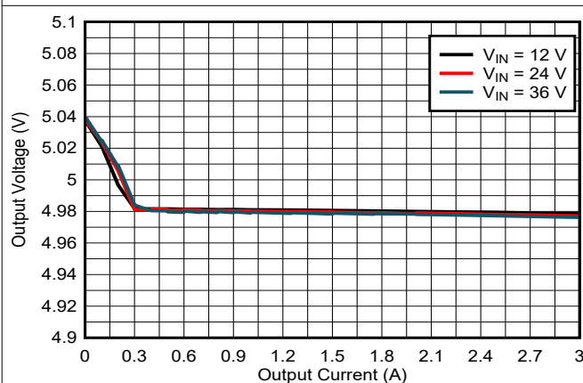
図 8-4. Load Regulation, V_{OUT} = 5\text{ V} , PFM Mode
