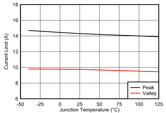
図 6-4. High-Side (Peak) and Low-Side (Valley) Current Limits TPSM63610
