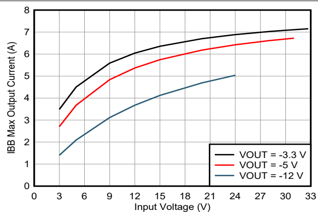
図 8-15. IBB Maximum Output Current
