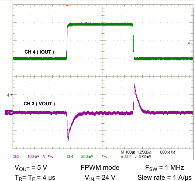
FIG 8-7. Load Transient, 4 A to 8 A, 1 A/μs
