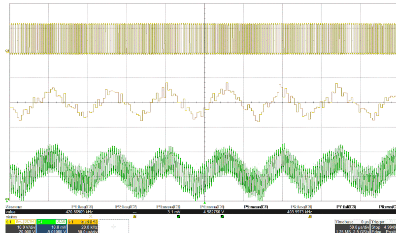
図 7-3. Output Ripple Without Ripple Cancellation Showing V_{\text{sw}} (Top), F_{\text{sw}} (Middle), V_{\text{out}} (Bottom)
