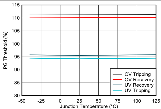
図 6-7. Power-Good (PG) Thresholds
