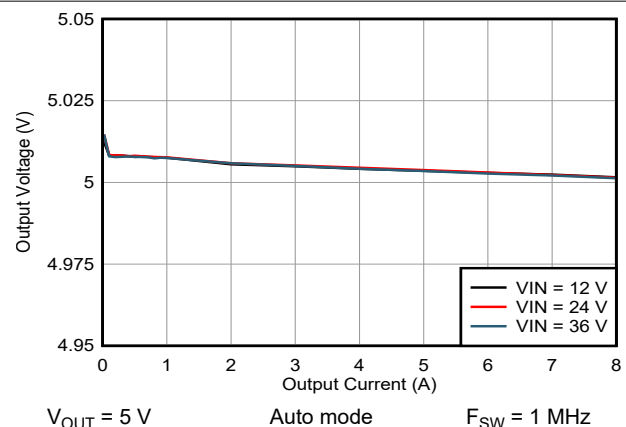
FIG 8-5. Load Regulation for V_{OUT} = 5\text{ V}
