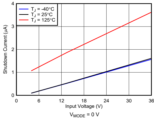
図 6-1. Shutdown Supply Current
