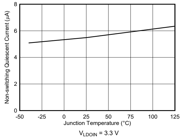
図 6-2. Non-Switching Input Supply Current
