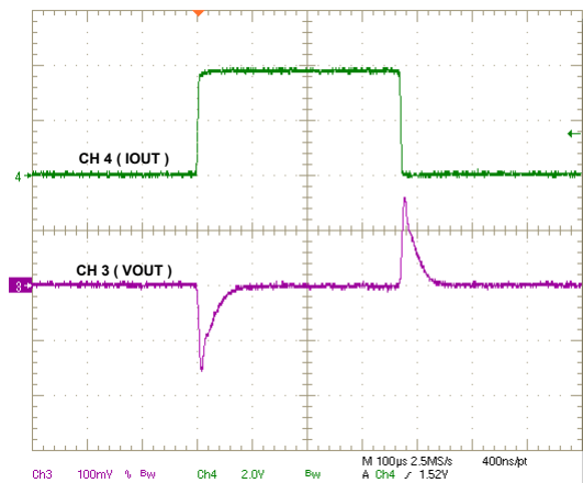
8-8. Load Transient, 0 A to 4 A, 1 A/μs
