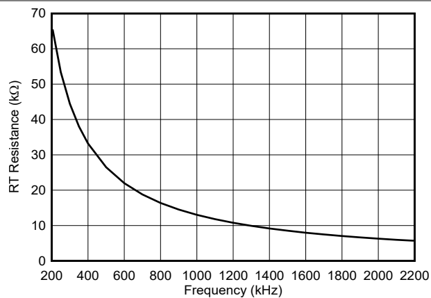
図 6-8. Switching Frequency Set by RT Resistor
