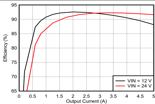
図 8-16. Efficiency for V_{OUT} = -12\text{ V} , FPWM Mode
