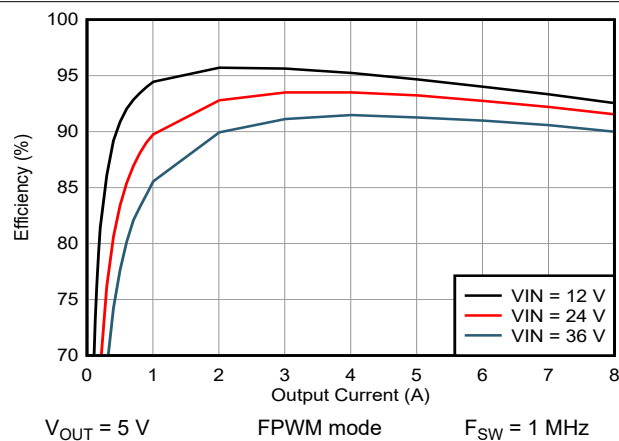
☒ 8-2. Efficiency for V_{OUT} = 5\text{ V}
