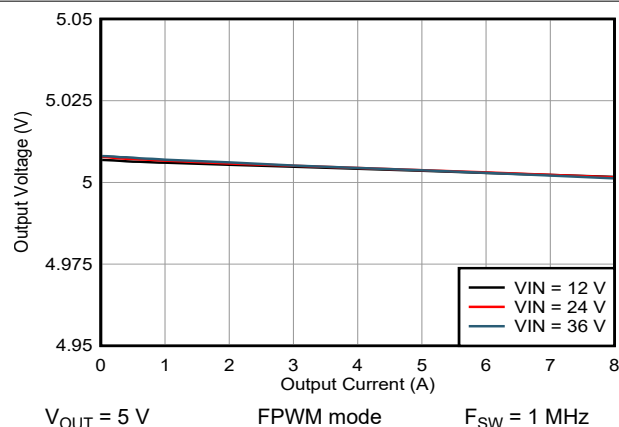
✎ 8-4. Load Regulation for V_{OUT} = 5\text{ V}
