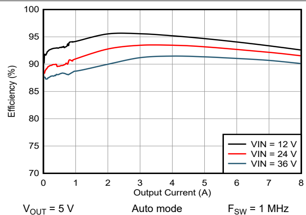
Fig. 8-3. Efficiency for V_{OUT} = 5\text{ V}
