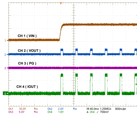
8-9. Start-up into Short Circuit
