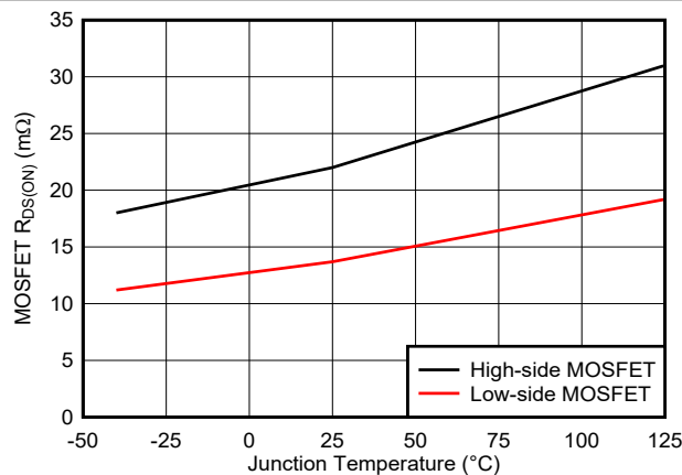
図 6-5. High-Side and Low-Side MOSFET R_{DS(on)}
