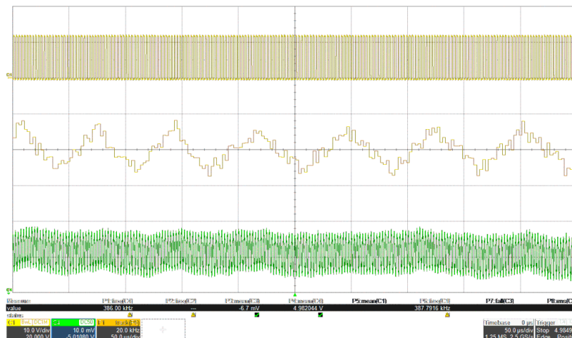
図 7-4. Output Ripple with Ripple Cancellation Showing V_{SW} (Top), F_{SW} (Middle), V_{OUT} (Bottom)
