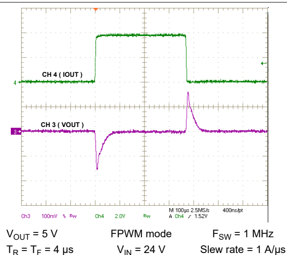
9-7. Load Transient, 0 A to 4 A, 1 A/μs
