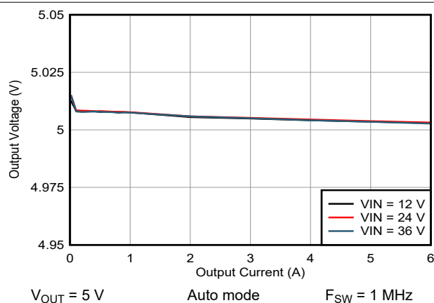
图 9-5. Load Regulation for V_{OUT} = 5\text{ V}
