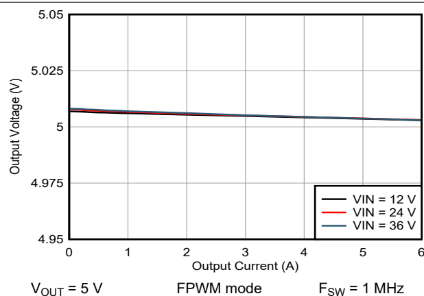
图 9-4. Load Regulation for V_{OUT} = 5\text{ V}
