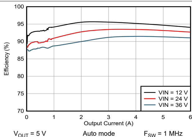
图 9-3. Efficiency for V_{OUT} = 5\text{ V}
