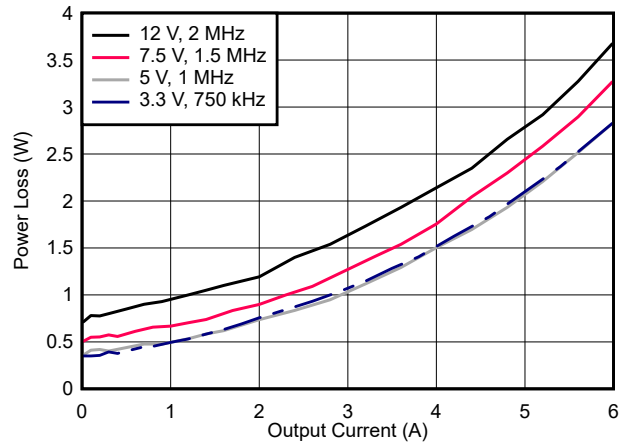
7-15. Power Dissipation
