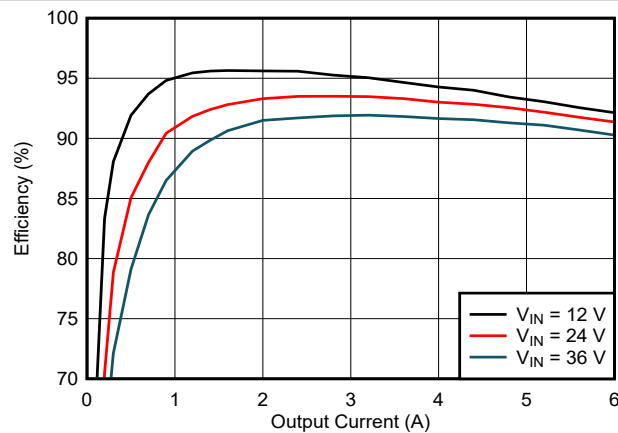
FIG 9-2. Efficiency
