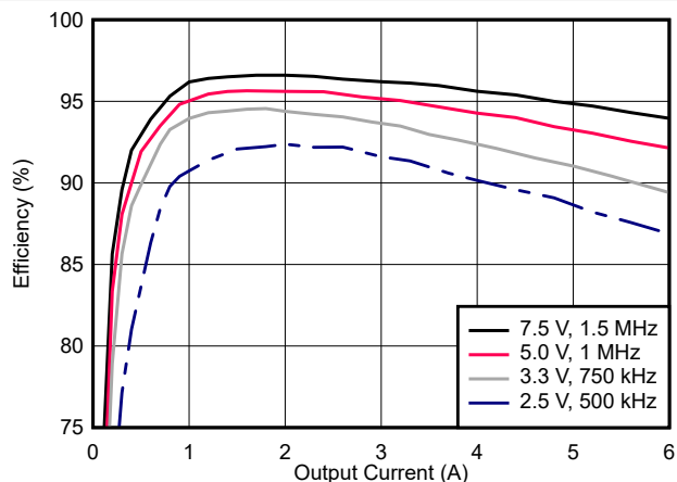
Figure 7-9. Efficiency
