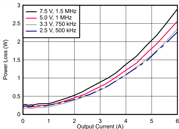
Figure 7-10. Power Dissipation
