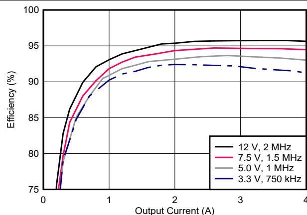
7-14. Efficiency
