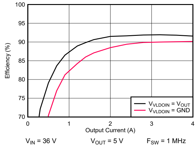
8-6. Efficiency Increase With External Bias
