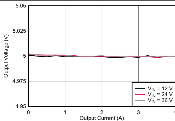
9-3. Load Regulation
