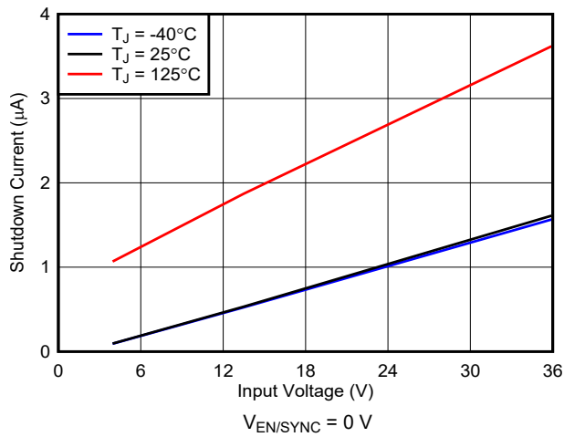
7-1. Shutdown Supply Current
