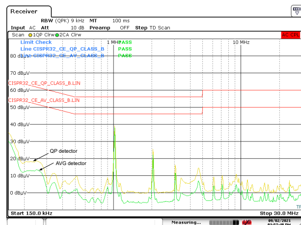
9-7. CISPR 32 Class B Conducted Emissions: V_{IN} = 24\text{ V}
