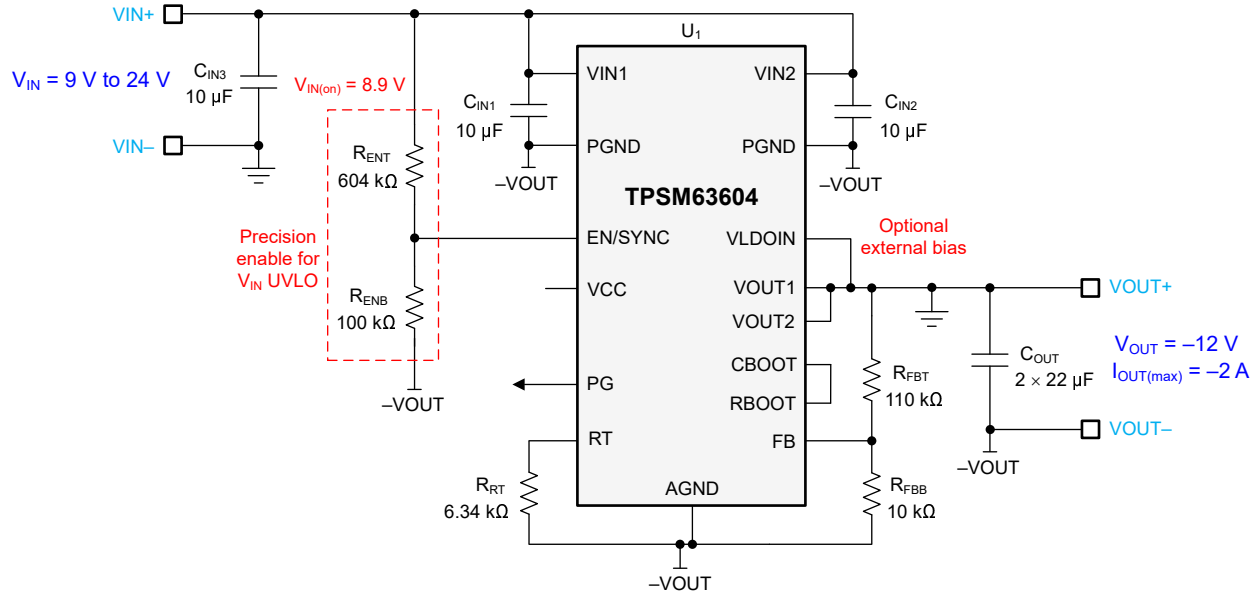
Figure 9-10. Circuit Schematic
