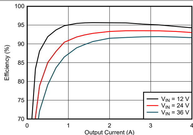
9-2. Efficiency
