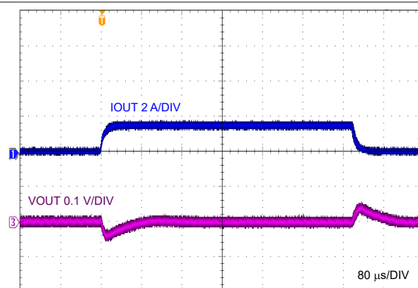
Figure 9-14. Load Transient, 0 A to 1.5 A
