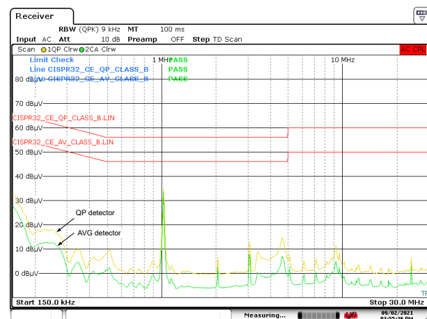
9-6. CISPR 32 Class B Conducted Emissions: V_{IN} = 12\text{ V}
