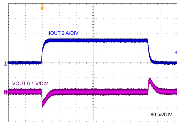
9-5. Load Transient, 0 A to 3 A, 1 A/ \mu s
