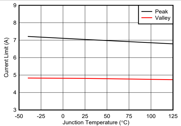
7-4. High-Side (Peak) and Low-Side (Valley) Current Limits
