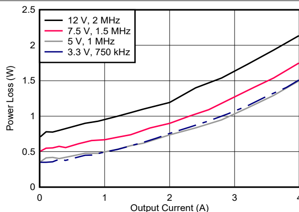
7-15. Power Dissipation
