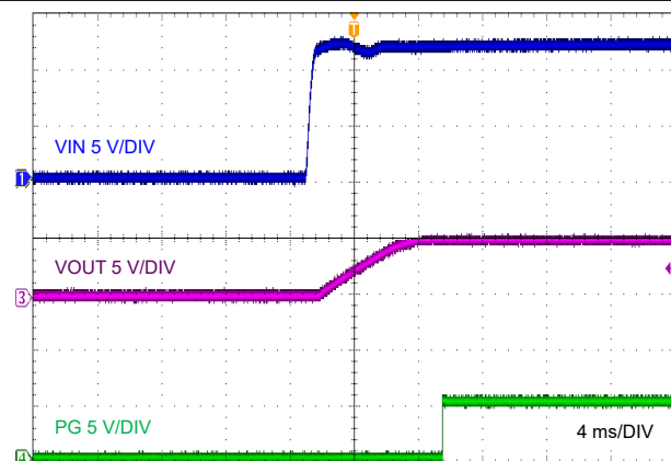
9-4. Start-Up, V_{IN} Stepped to 12 V
