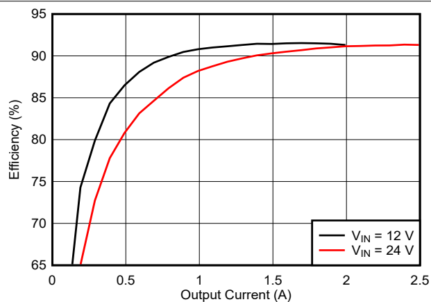
Figure 9-12. Efficiency
