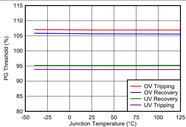
Figure 6-6. Power-Good (PG) Thresholds
