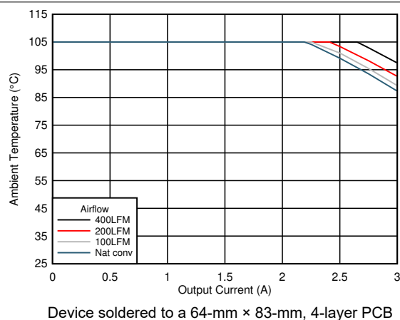
図 6-10. Safe Operating Area V_{OUT} = 1.8\text{ V} , F_{SW} = 600\text{ kHz}
