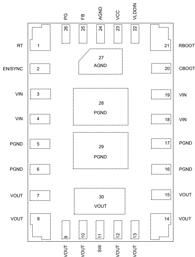
图 5-1. 30-Pin QFN, RDH Package (Top View)
