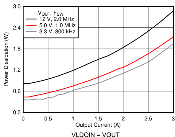
Figure 6-20. Power Dissipation
