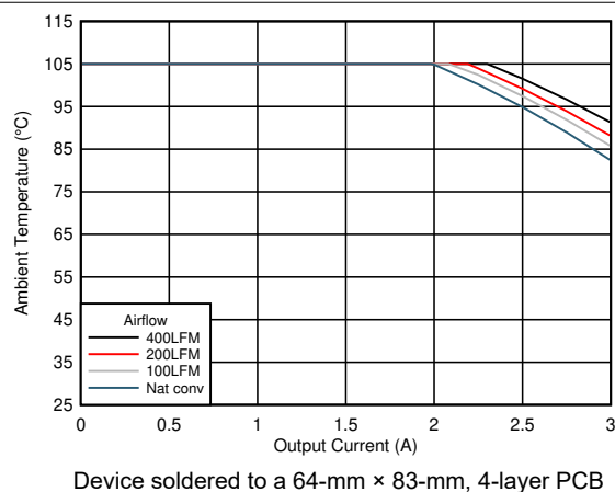
図 6-12. Safe Operating Area V_{OUT} = 5.0\text{ V} , F_{SW} = 1\text{ MHz}
