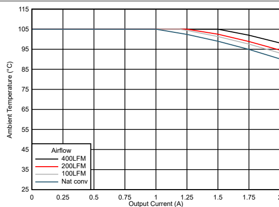
Figure 7-16. Safe Operating Area ( V_{OUT} = 12\text{ V} )
