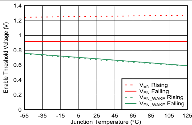
7-5. Enable Thresholds
