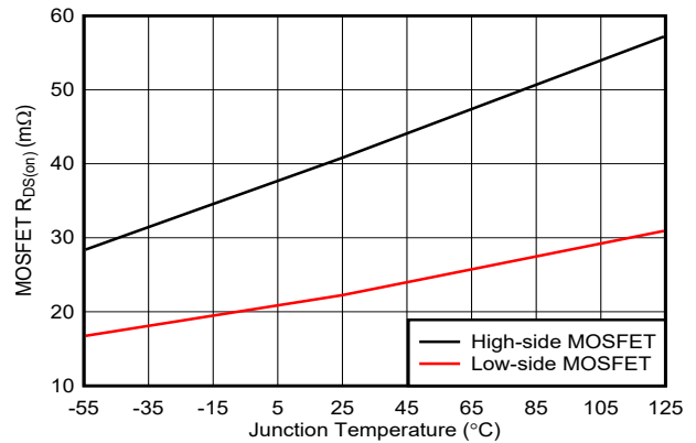
7-4. High-Side and Low-Side MOSFET R_{DS(on)}
