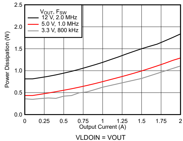
7-18. Power Dissipation
