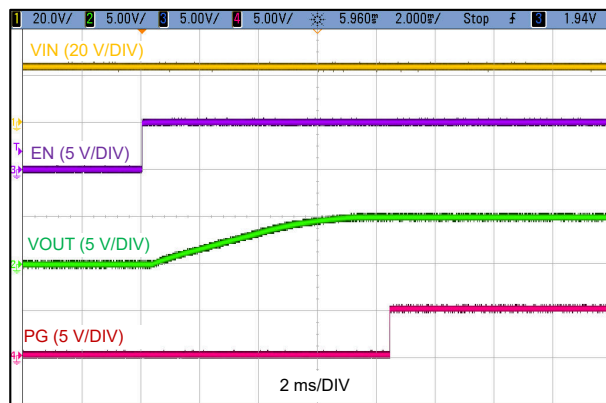
9-2. Start-Up Waveforms
