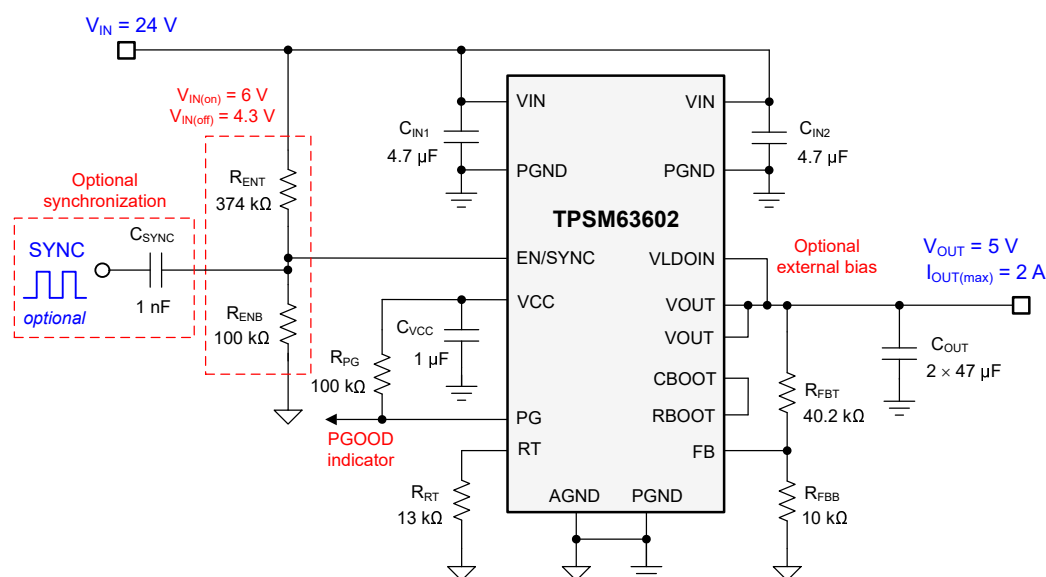
Figure 9-1. Circuit Schematic
