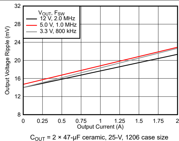
7-19. Output Voltage Ripple
