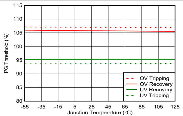
7-6. Power-Good (PG) Thresholds
