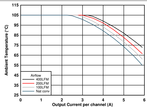
6-4. Safe Operating Area (VOUT = 1.2 V)
