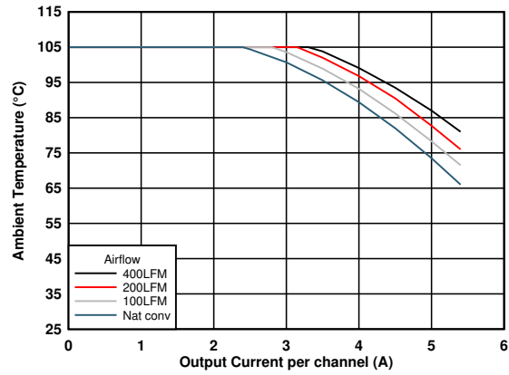
6-14. Safe Operating Area (VOUT = 3.3 V)
