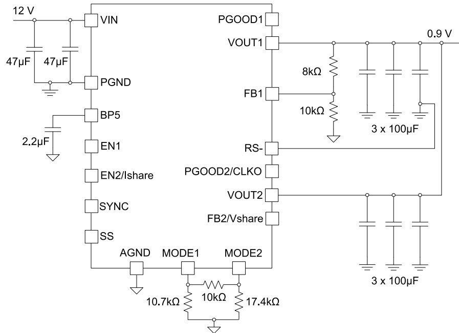
8-2. TPSM5D1806 Parallel Outputs Typical Schematic
