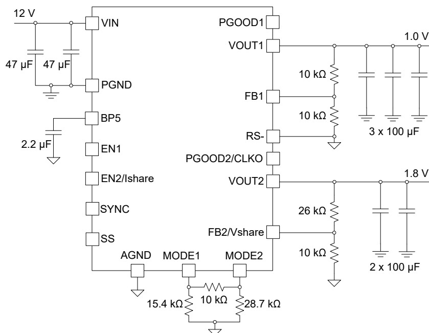
8-1. TPSM5D1806 Dual Output Typical Schematic
