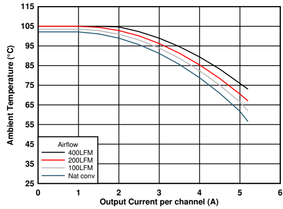
6-7. Safe Operating Area (VOUT = 5 V)
