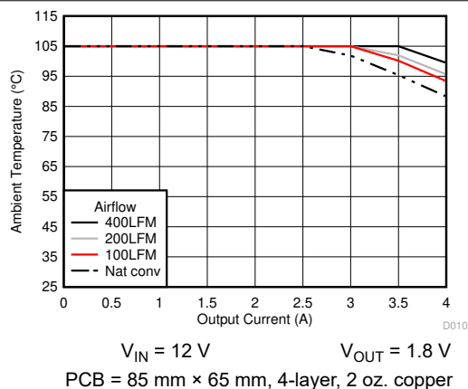
Figure 6-11. Safe Operating Area
