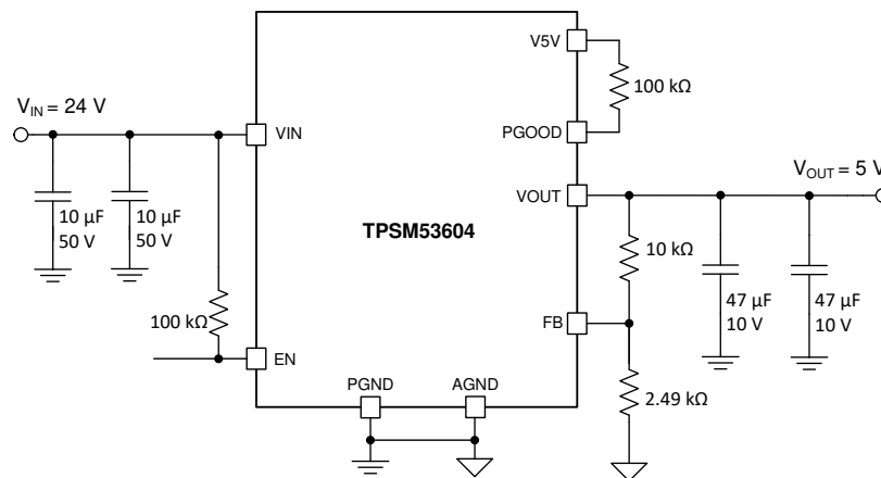
图 8-1. TPSM53604 Typical Schematic
