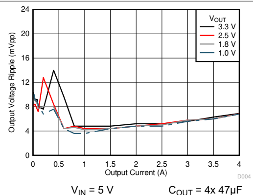
6-4. Voltage Ripple versus Output Current
