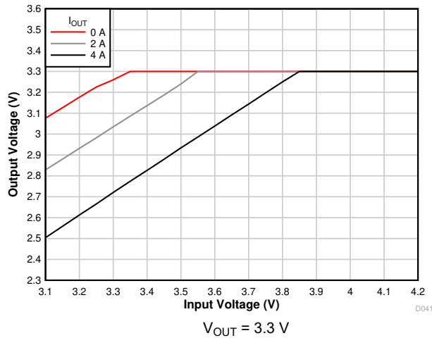
7-7. Voltage Dropout
