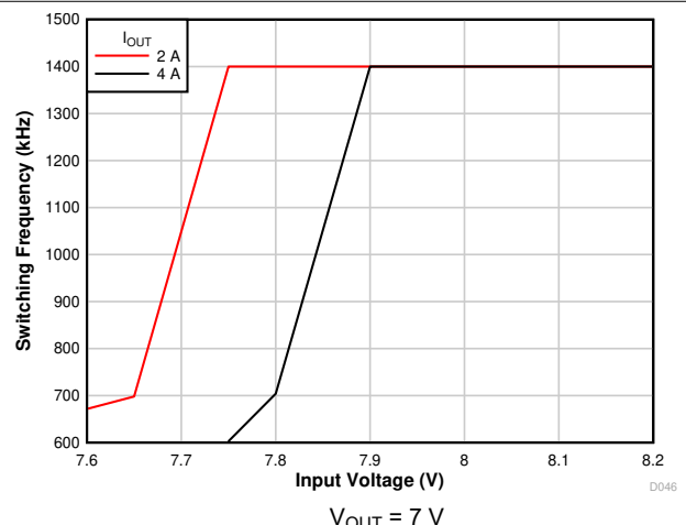
7-12. Frequency Foldback
