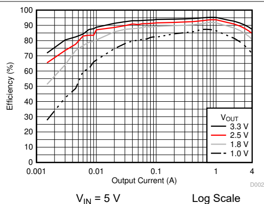
6-2. Efficiency versus Output Current
