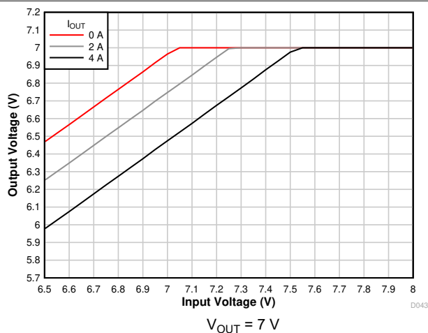
7-11. Voltage Dropout
