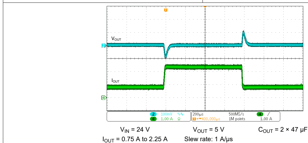
8-4. Transient Response
