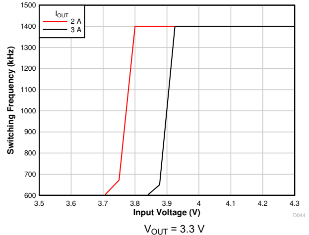
7-8. Frequency Foldback
