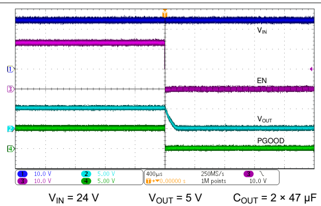
8-3. Enable Turn-OFF
